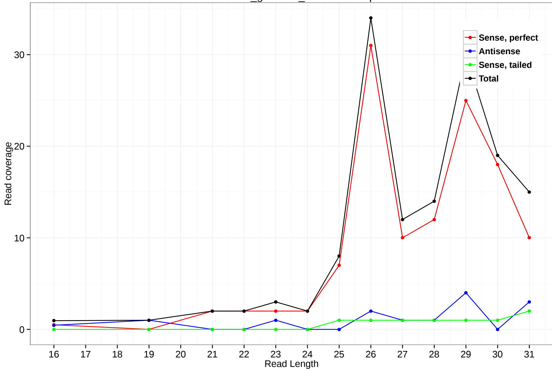
rheMac3_genscan_chr10.2092.5p
