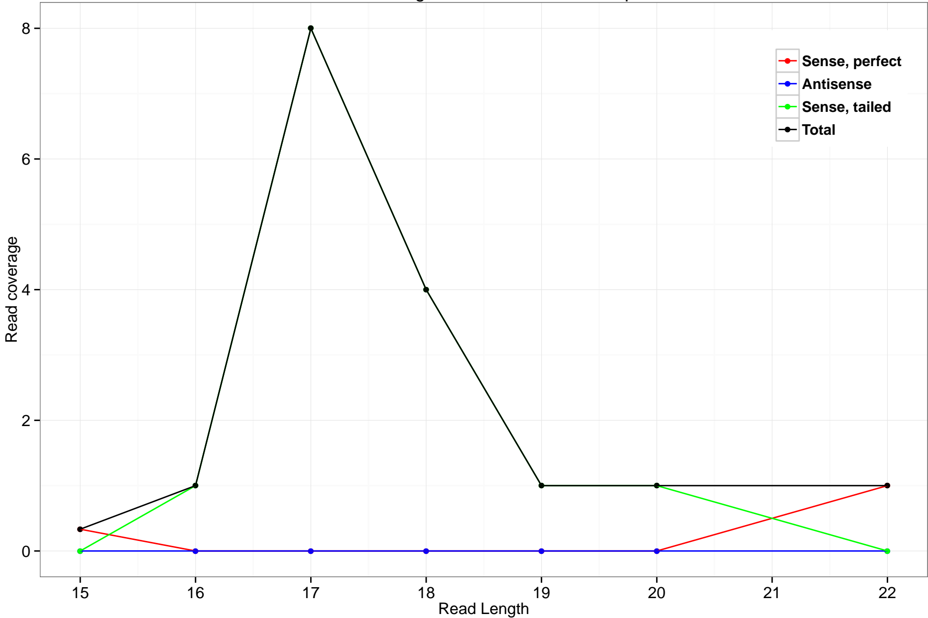
rheMac3_genscan_chr10.2044_3.5p
