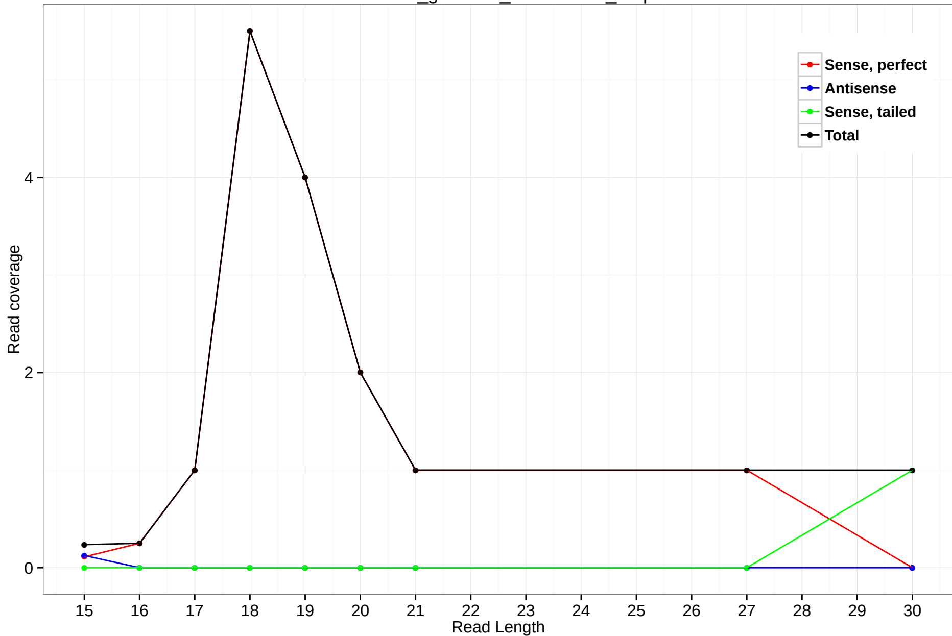
rheMac3_genscan_chr10.1965_0.5p
