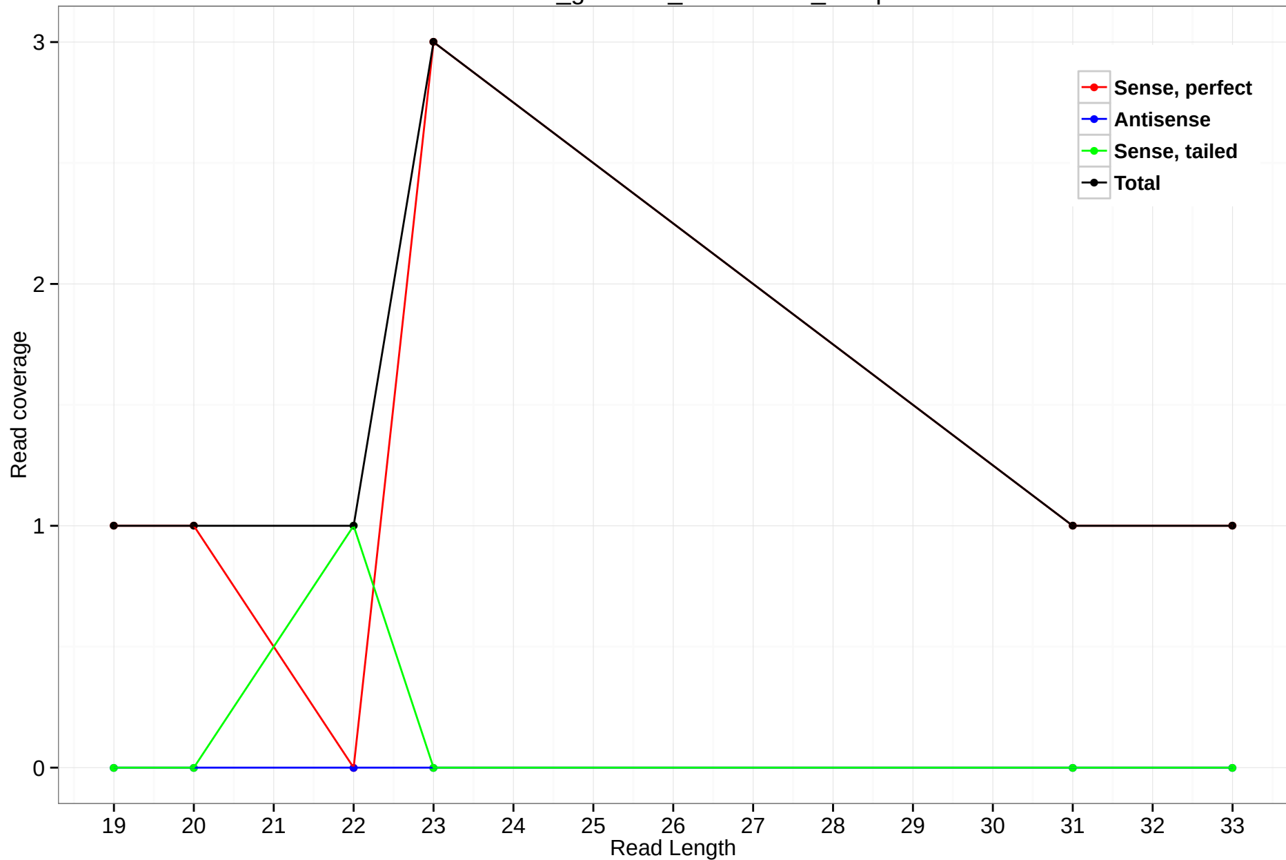
rheMac3_genscan_chr10.1962_13.5p
