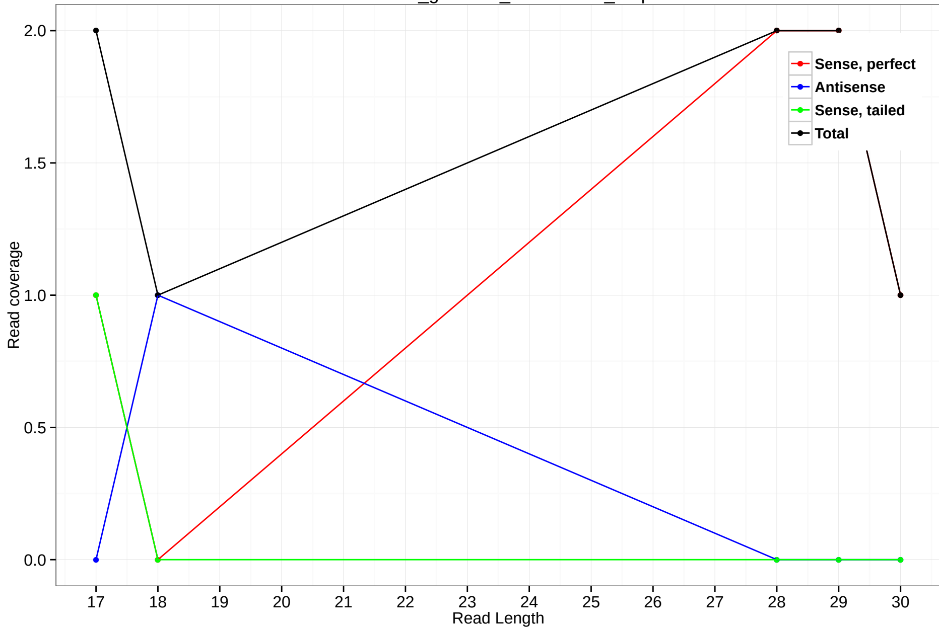
rheMac3_genscan_chr10.1931_0.5p
