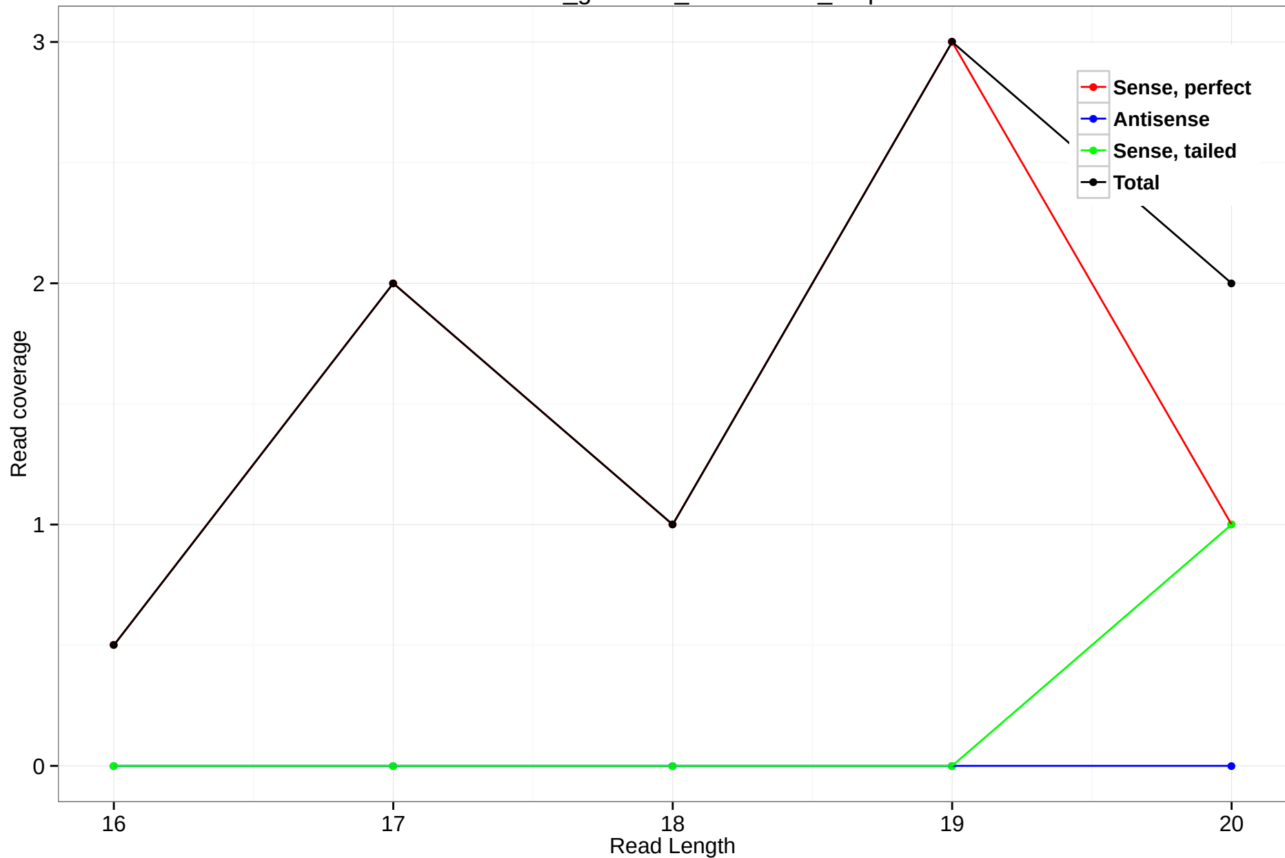
rheMac3_genscan_chr10.1922_0.3p
