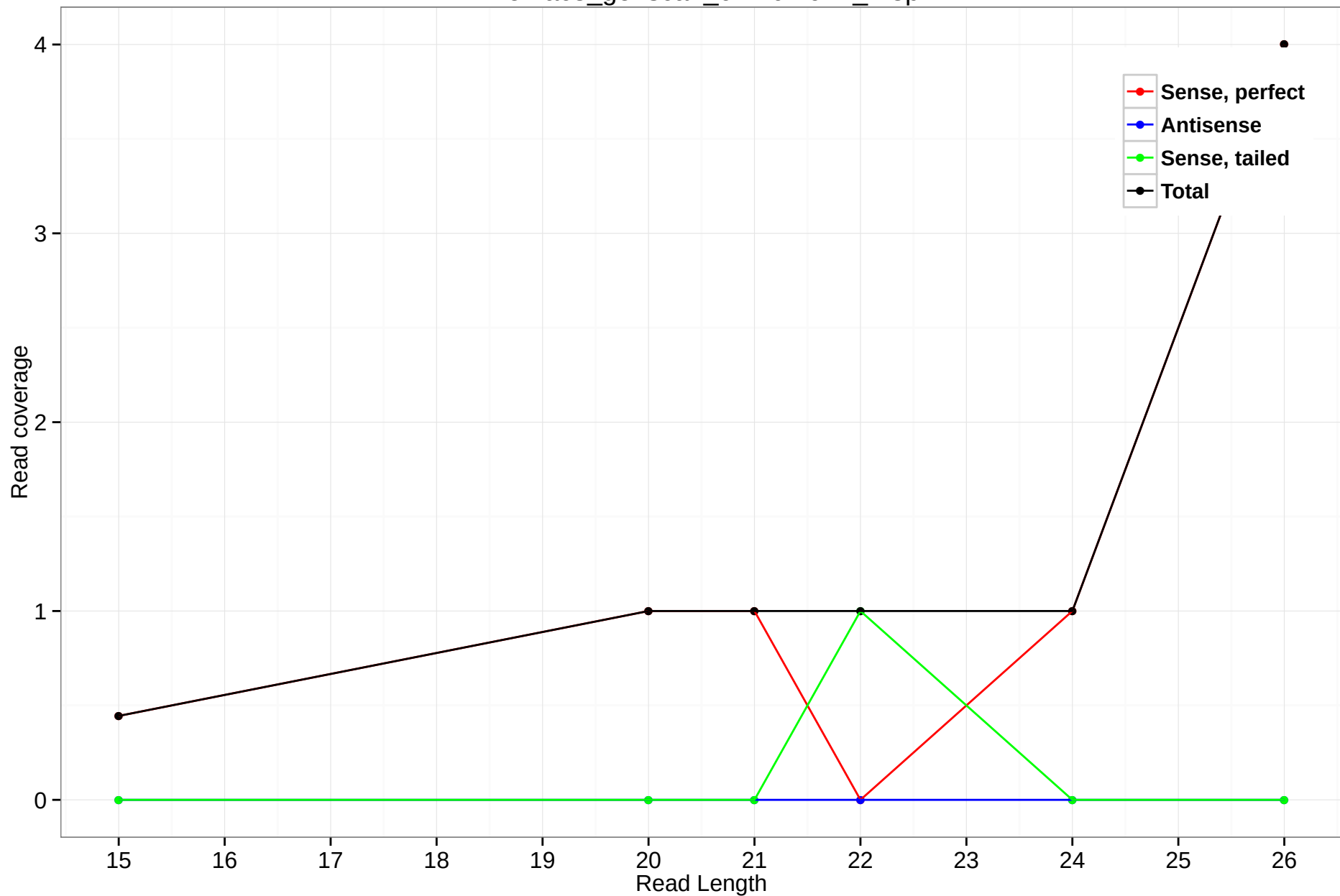
rheMac3_genscan_chr10.1914_1.3p
