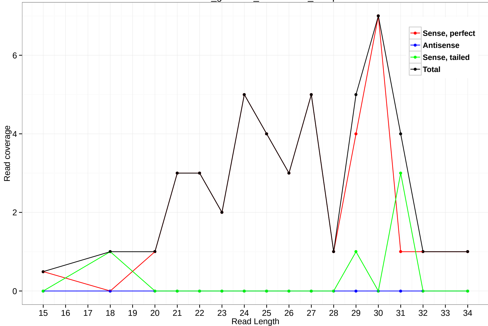
rheMac3_genscan_chr10.1888_13.3p
