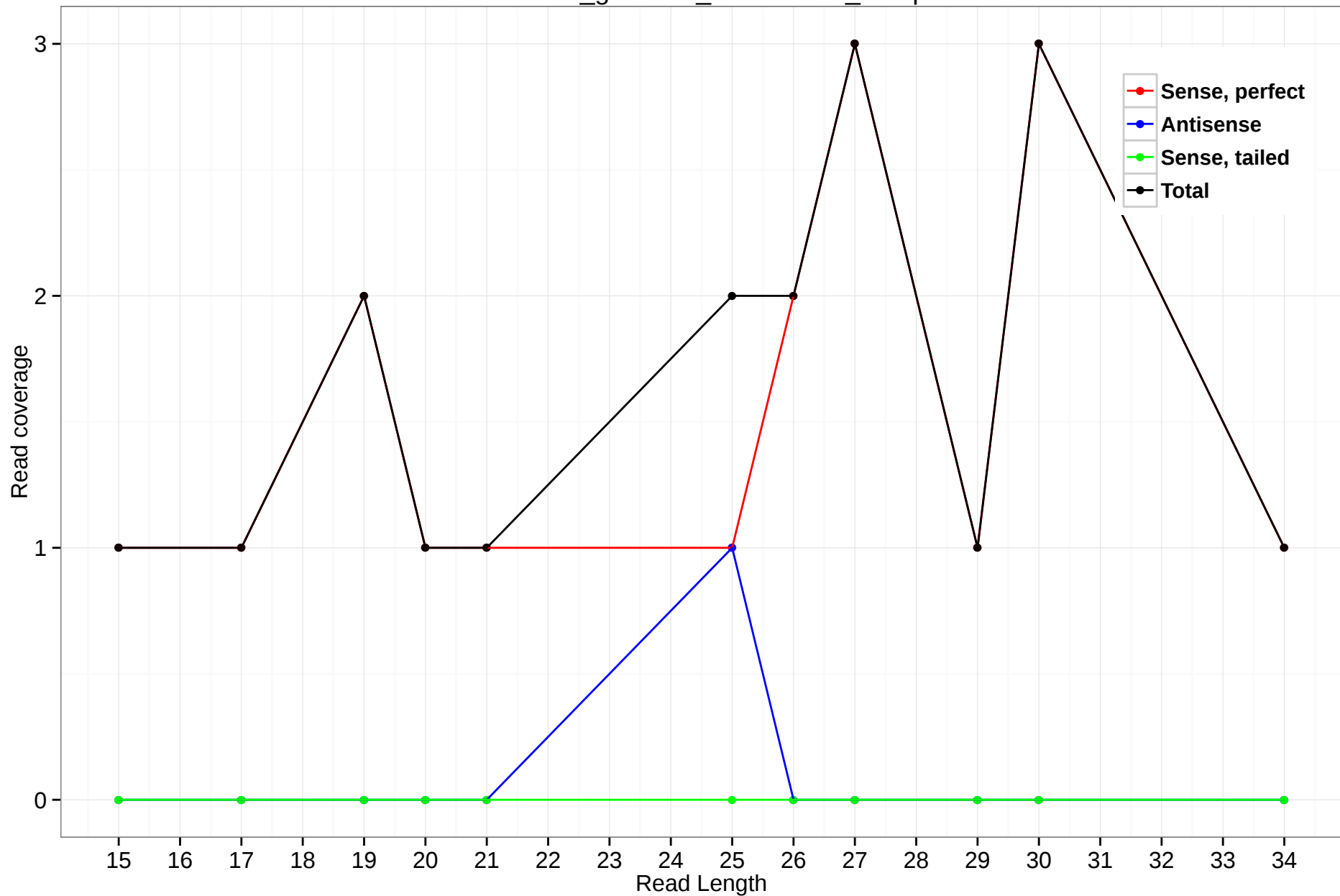
rheMac3_genscan_chr10.1888_12.5p
