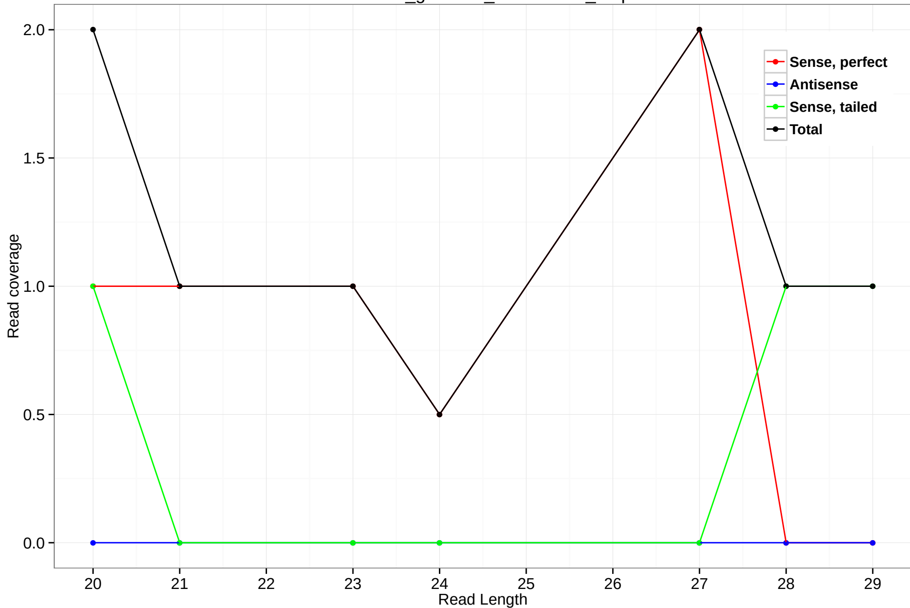
rheMac3_genscan_chr10.1888_0.3p
