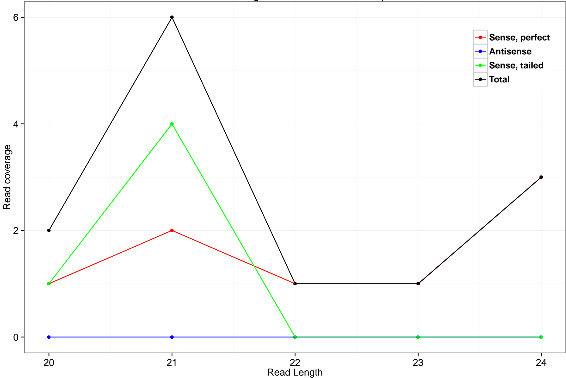
rheMac3_genscan_chr10.1884_8.3p
