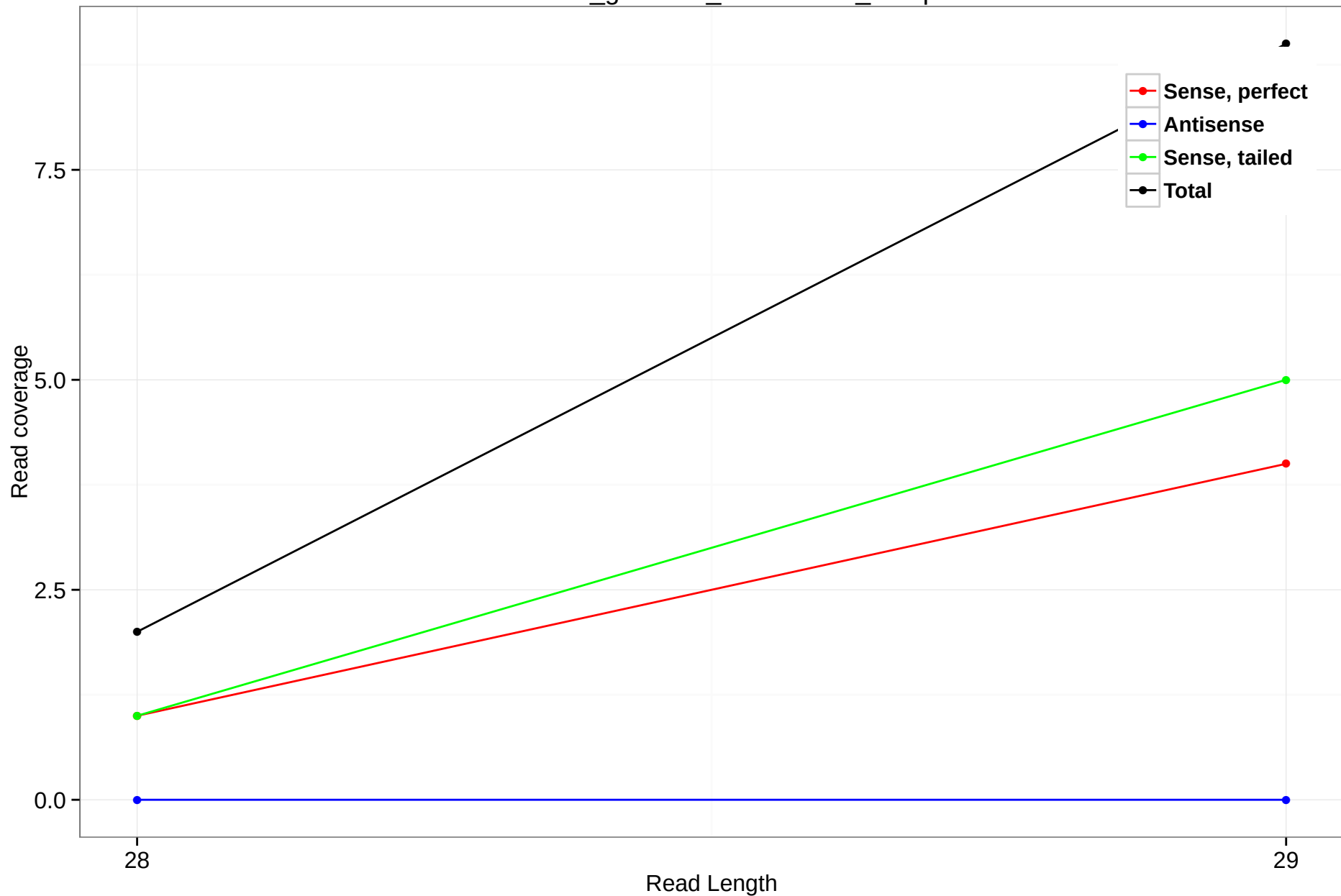
rheMac3_genscan_chr10.1867_11.3p
