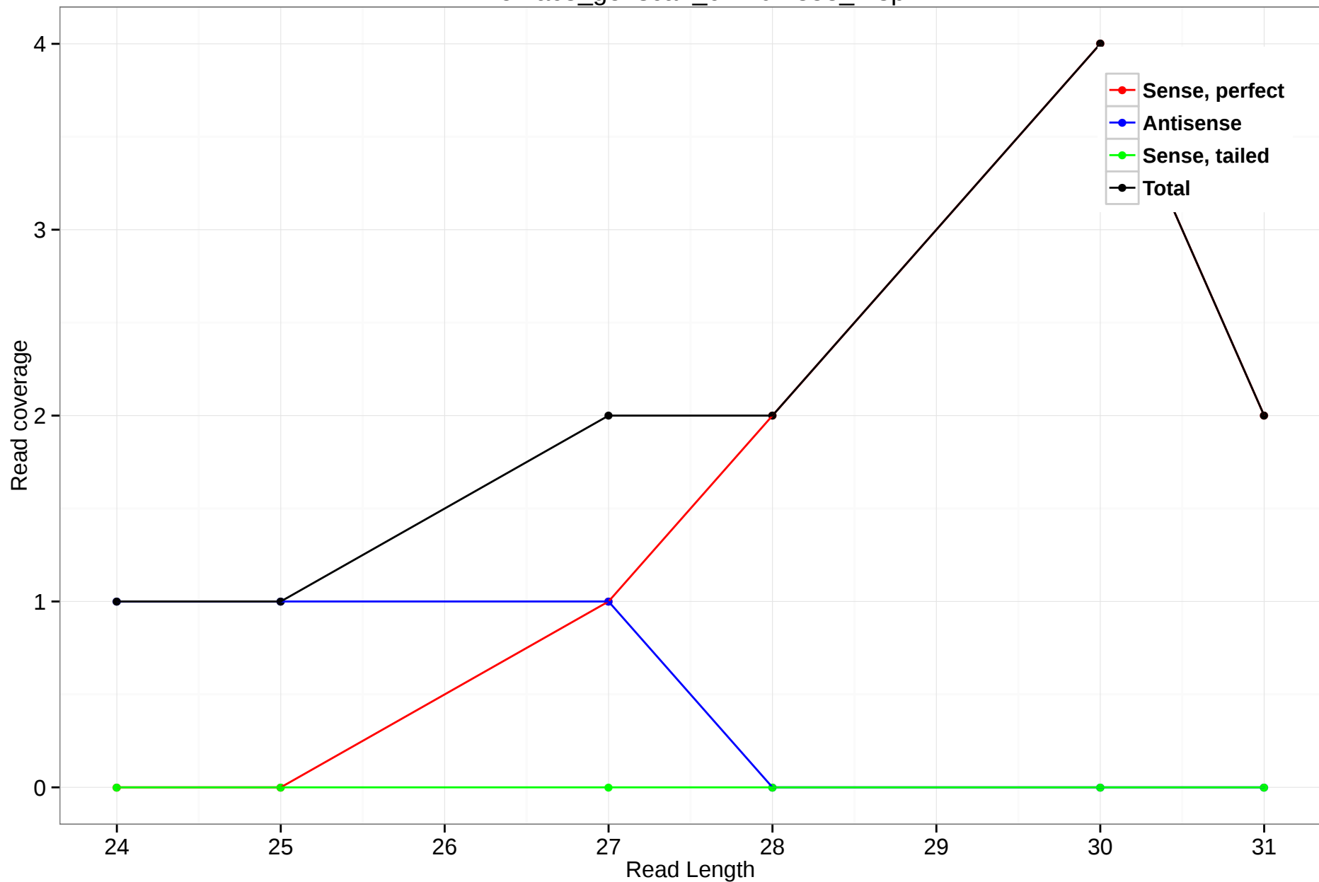
rheMac3_genscan_chr10.1858_1.3p
