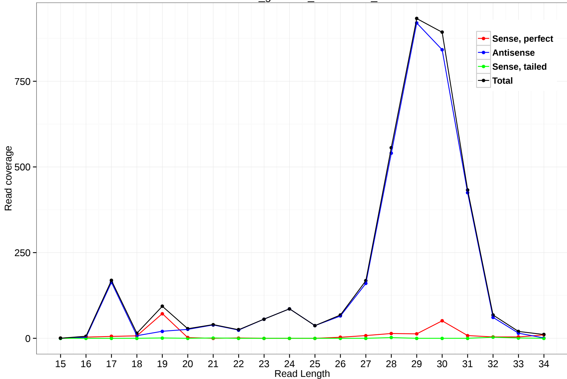
rheMac3_genscan_chr10.1856_22
