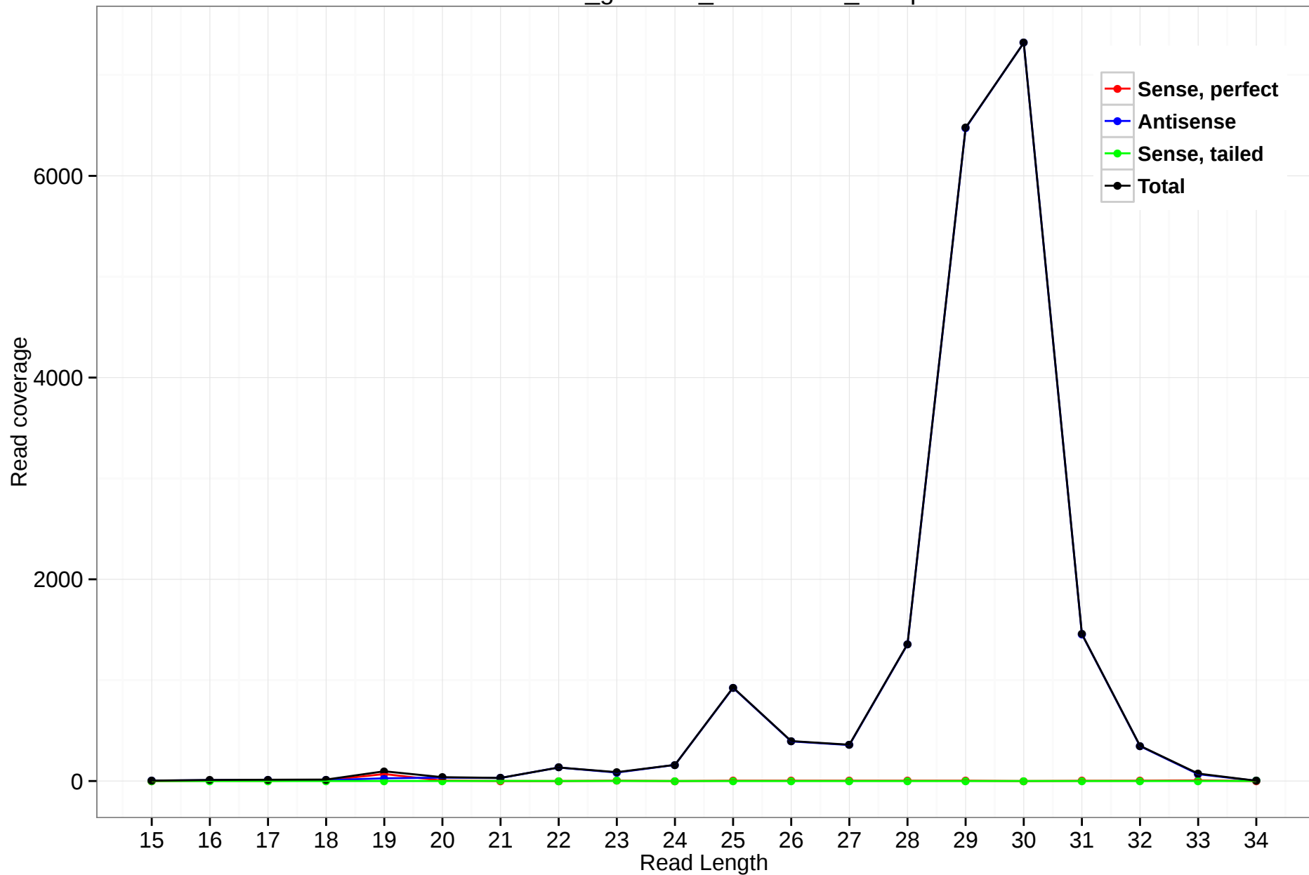
rheMac3_genscan_chr10.1856_19.3p
