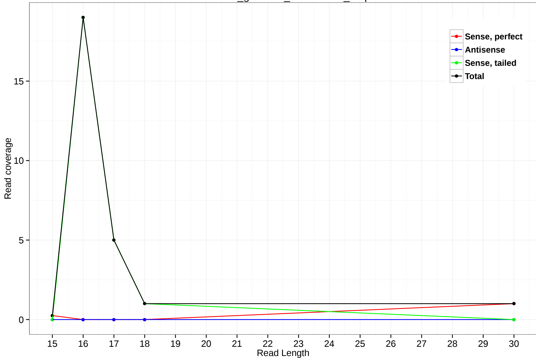
rheMac3_genscan_chr10.1829_1.5p
