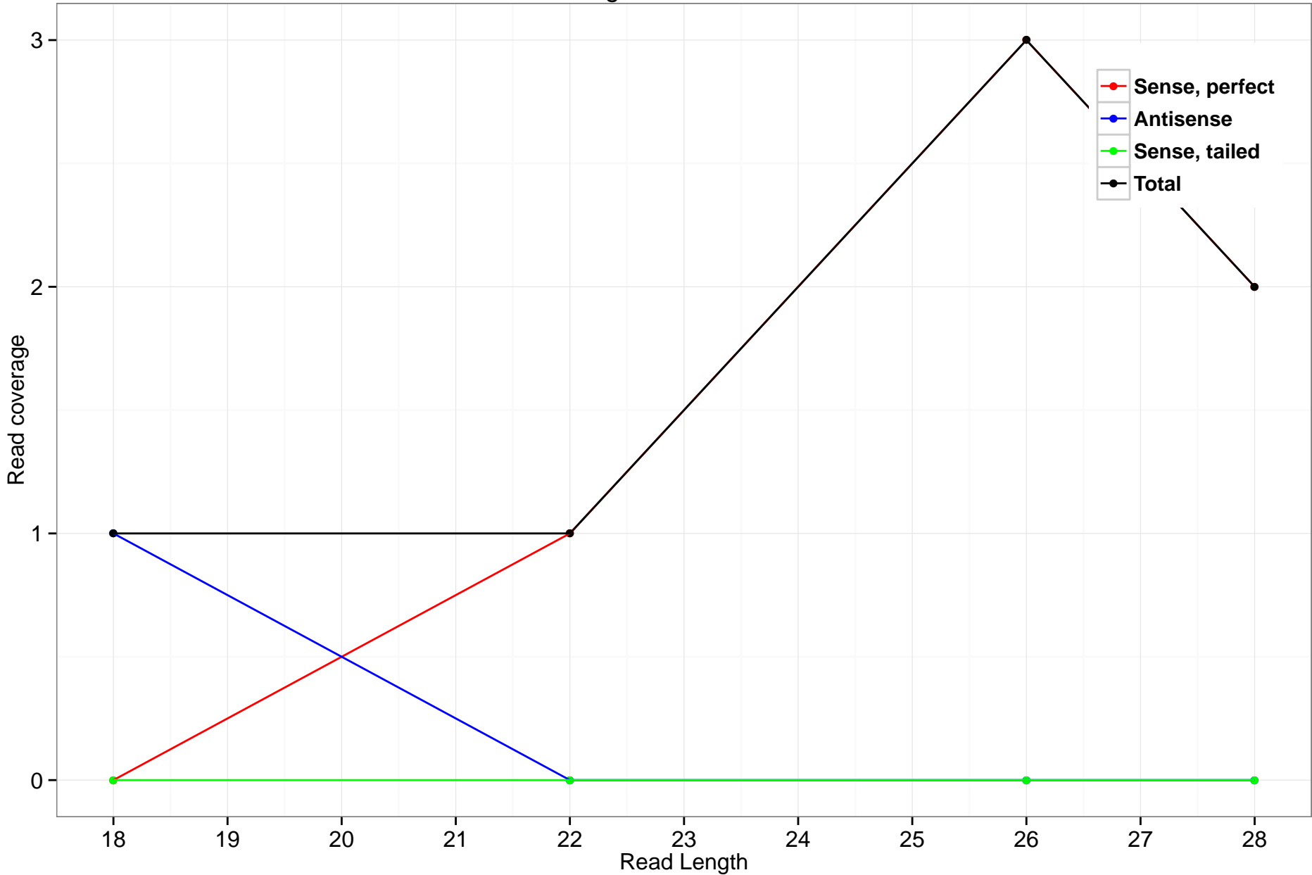
rheMac3_genscan_chr10.1816_7
