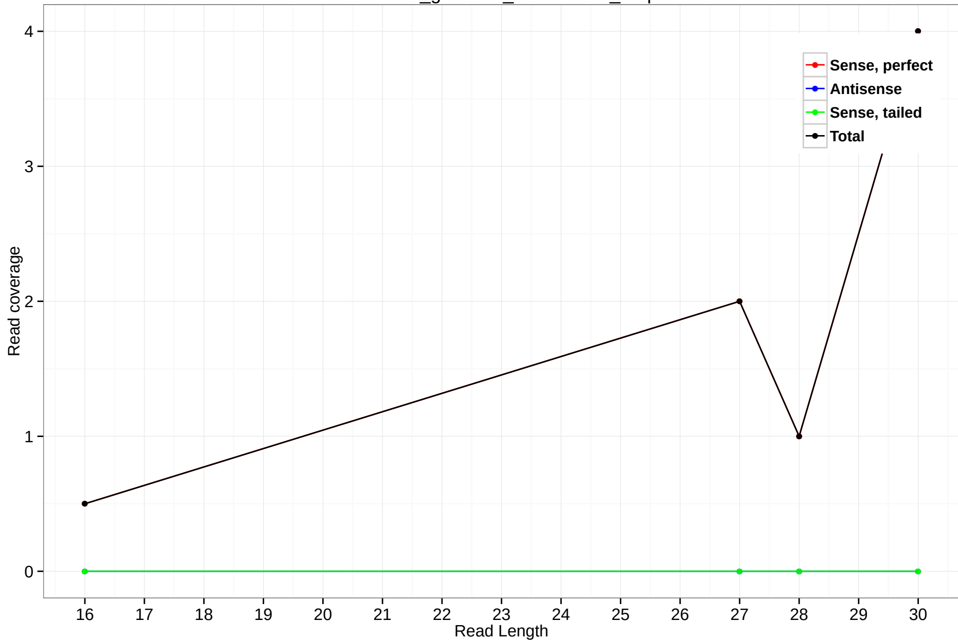
rheMac3_genscan_chr10.1778_3.5p
