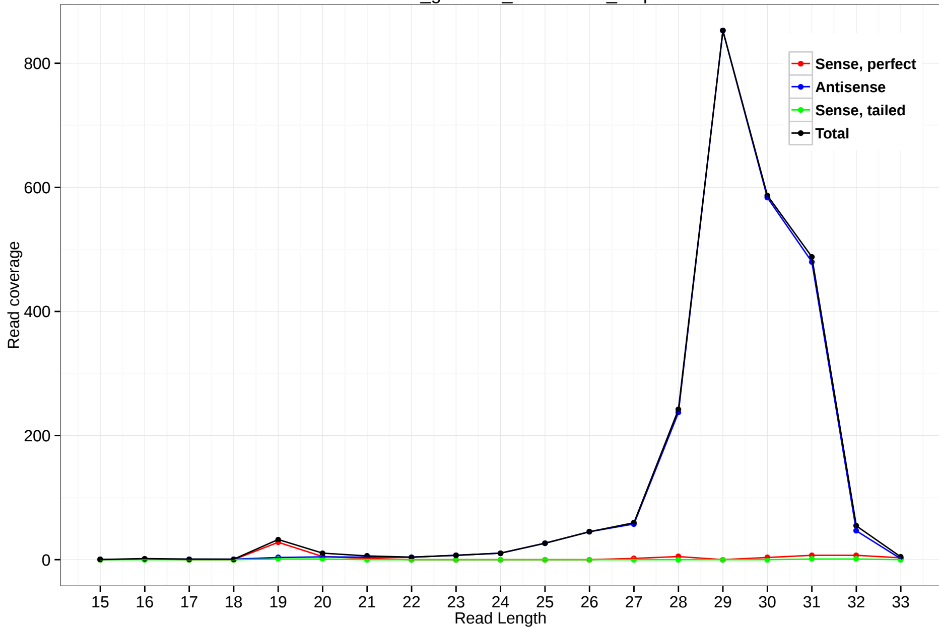
rheMac3_genscan_chr10.1731_7.5p
