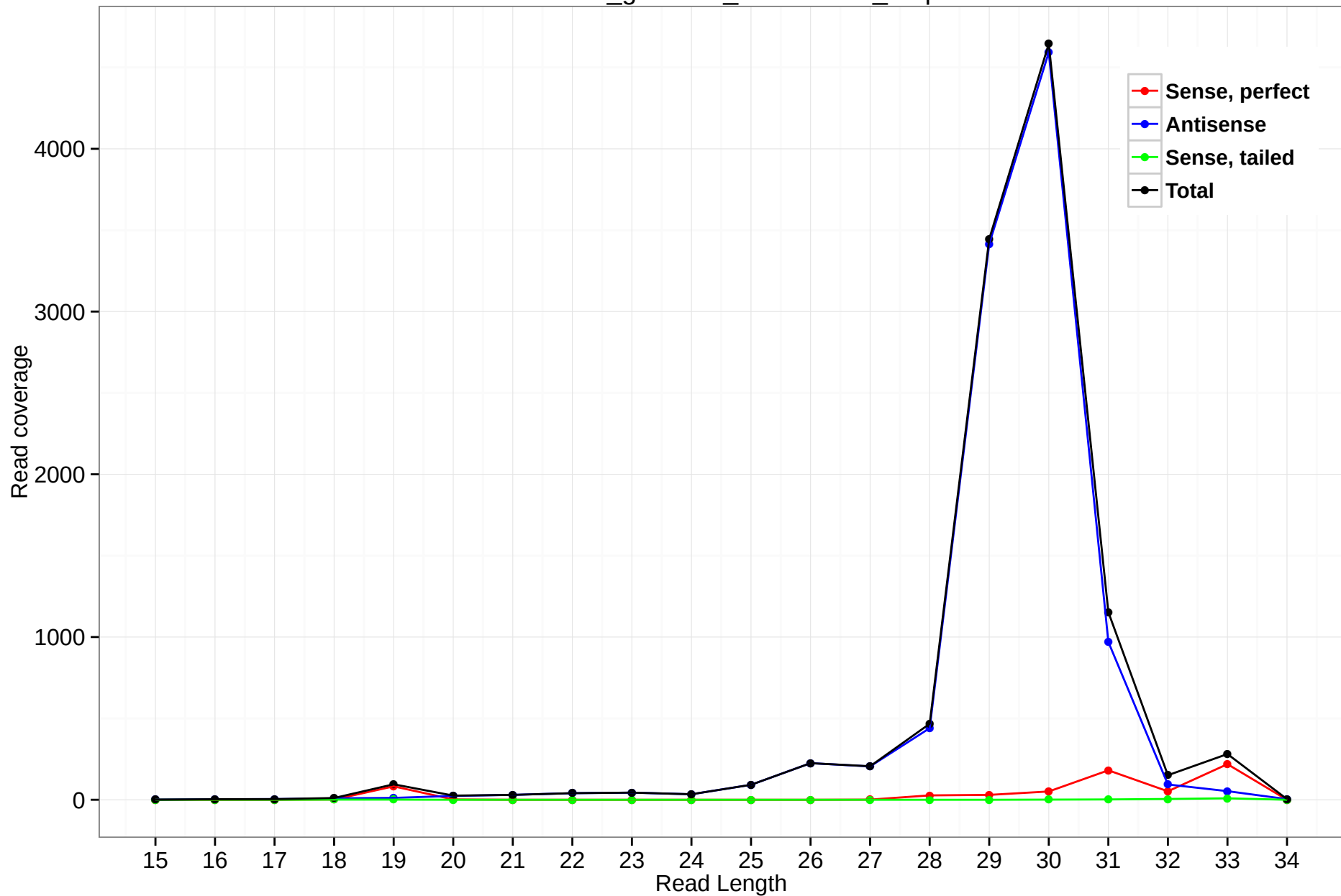
rheMac3_genscan_chr10.1731_5.3p
