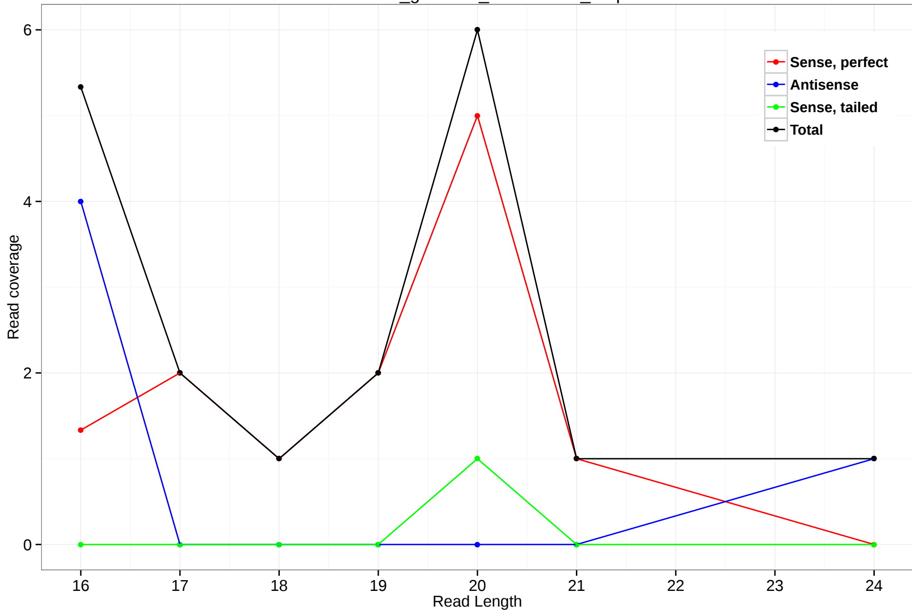
rheMac3_genscan_chr10.1716_0.5p
