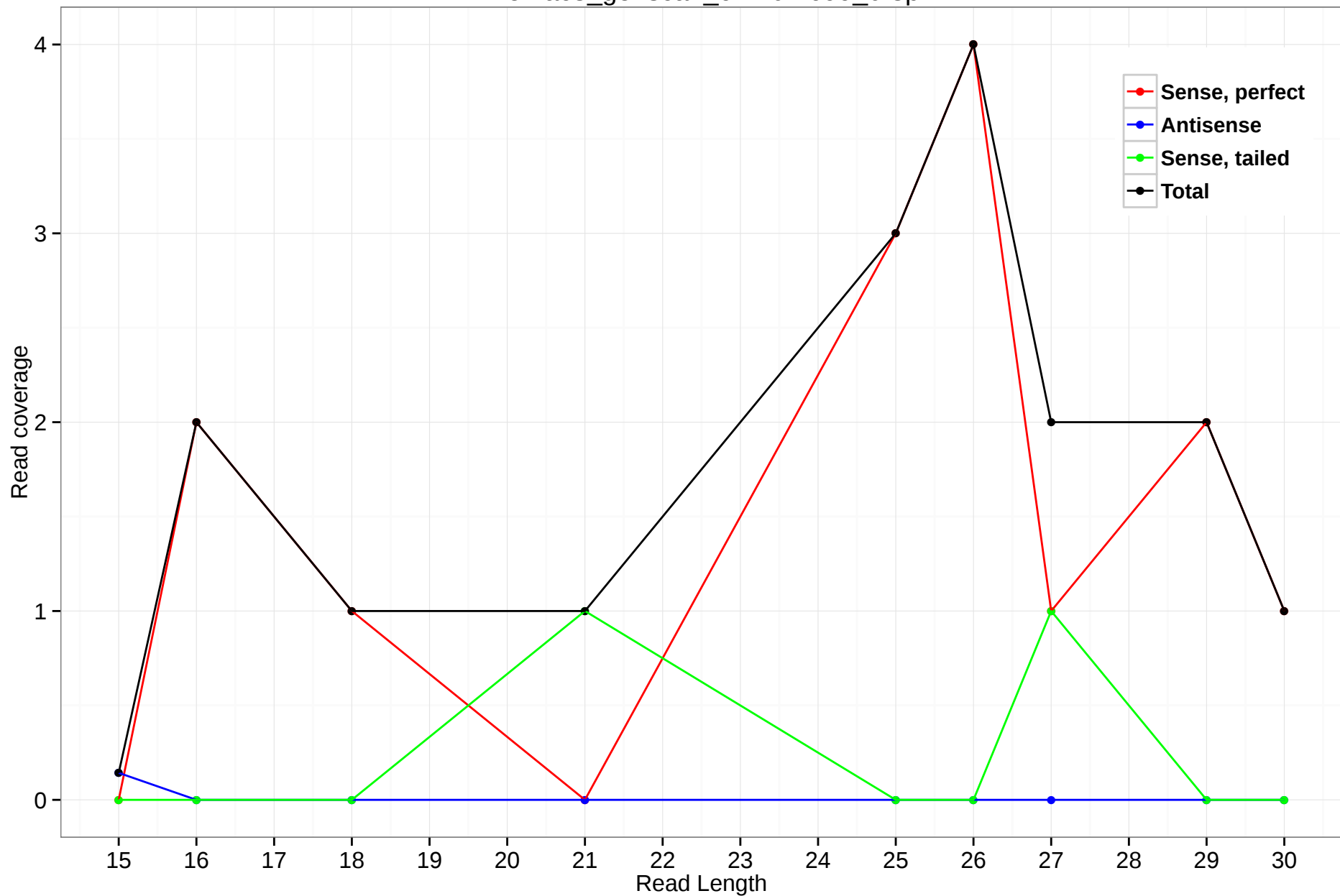
rheMac3_genscan_chr10.1699_0.3p
