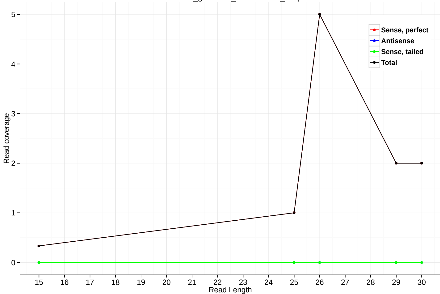
rheMac3_genscan_chr10.1691_4.5p
