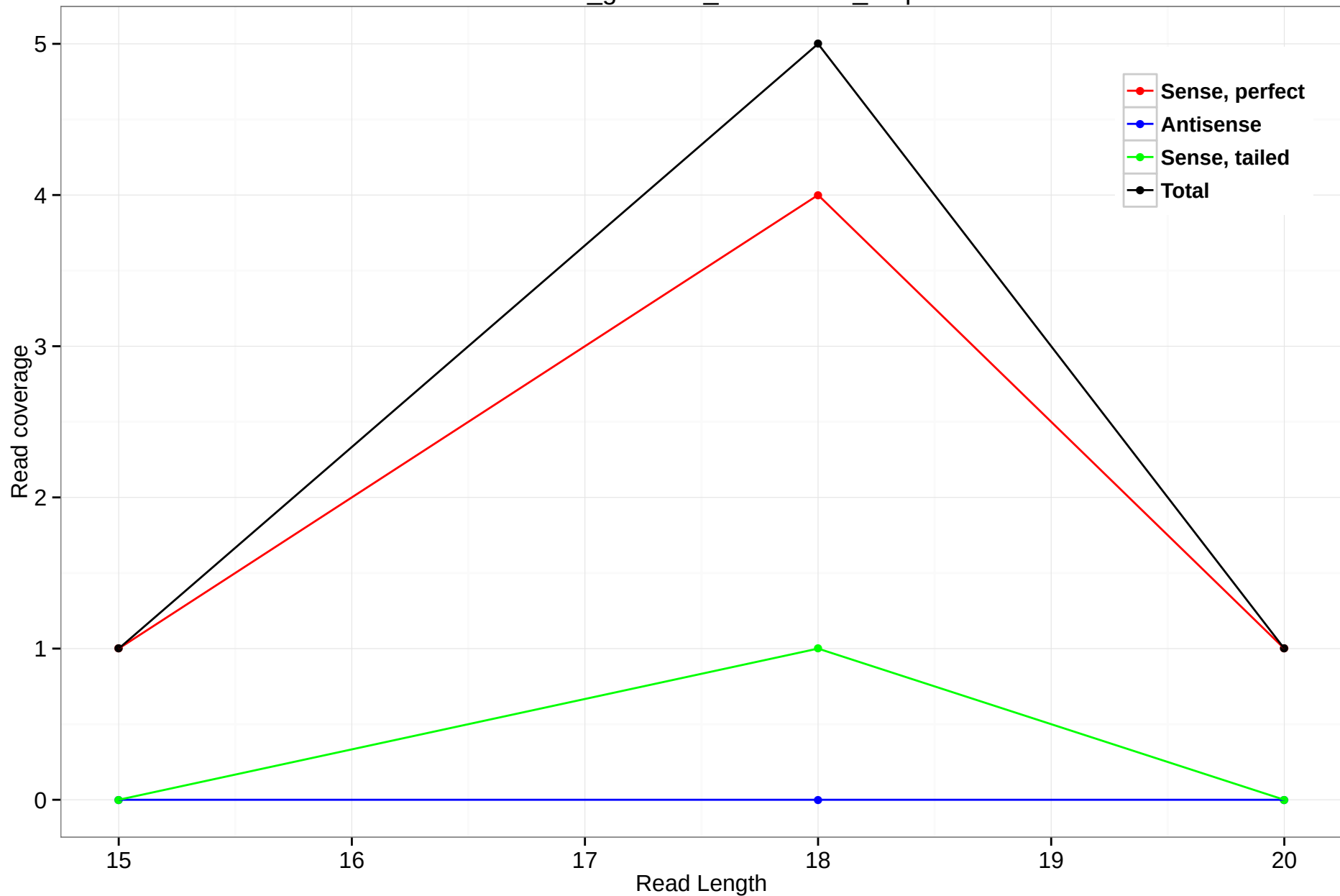
rheMac3_genscan_chr10.1691_0.5p
