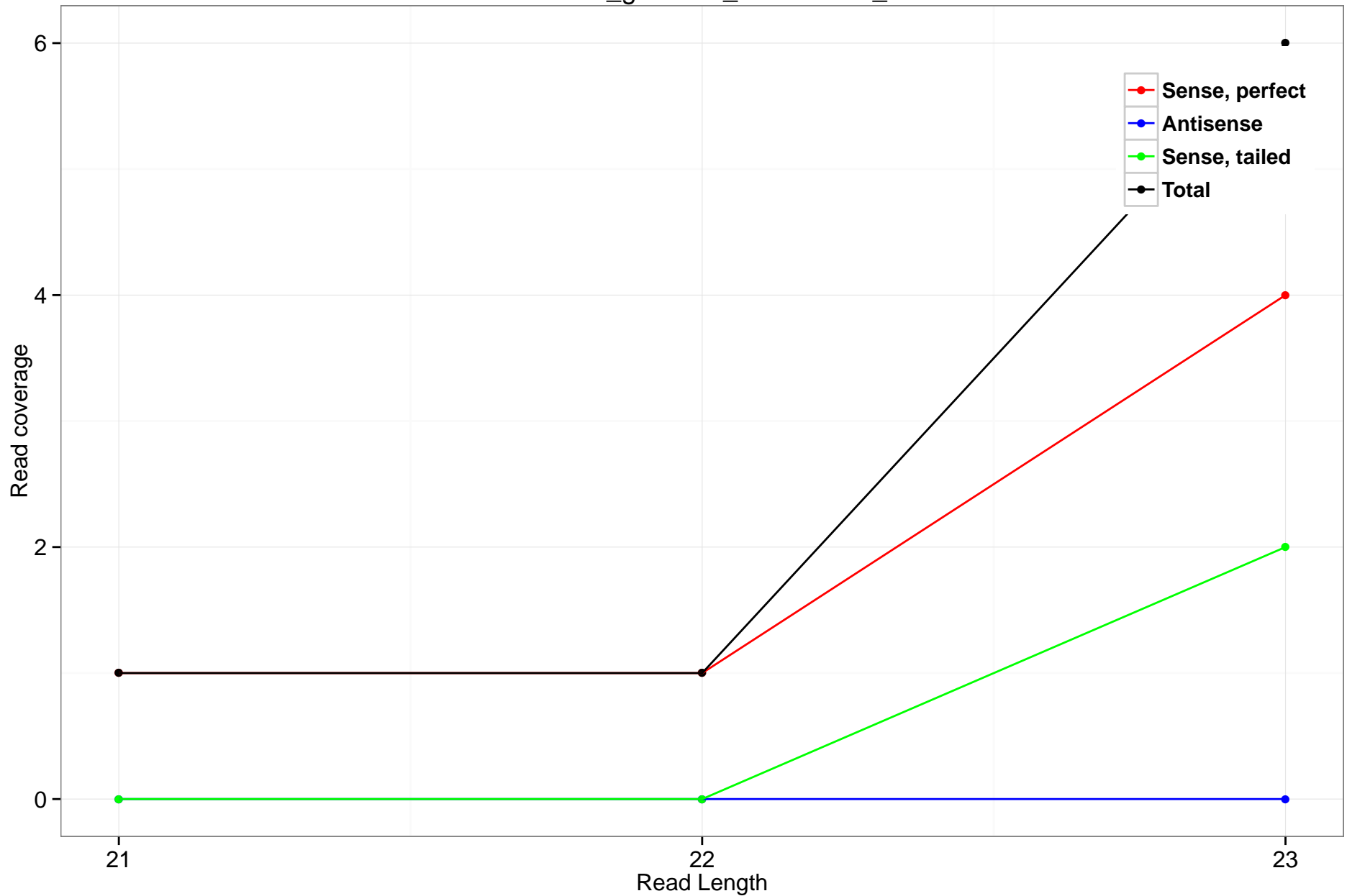
rheMac3_genscan_chr10.1690_7
