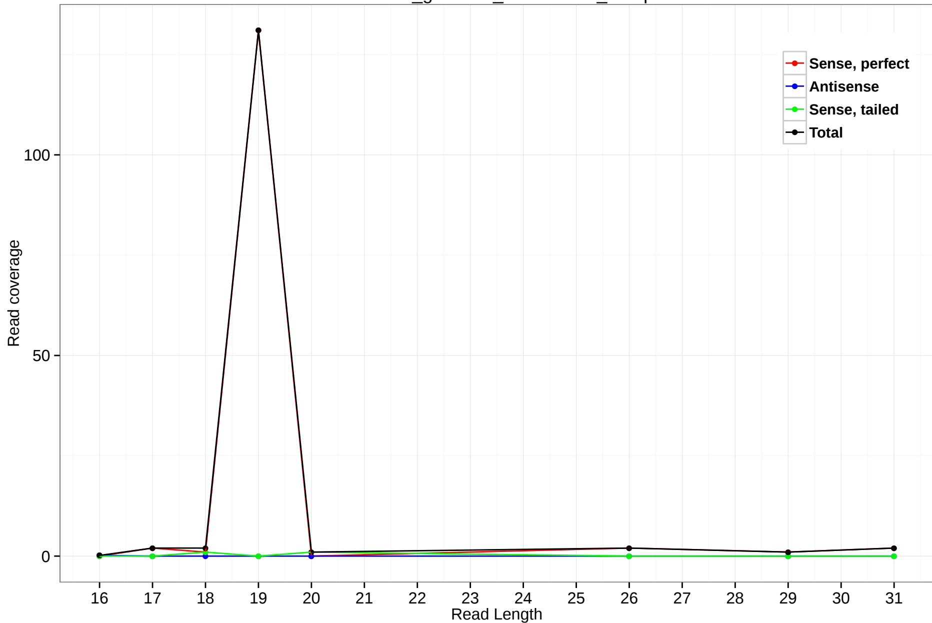
rheMac3_genscan_chr10.1675_12.3p
