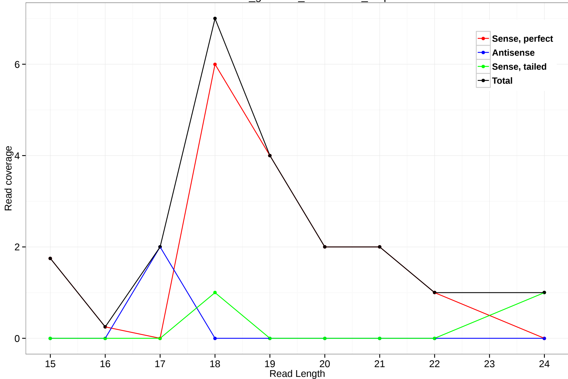
rheMac3_genscan_chr10.1661_9.3p
