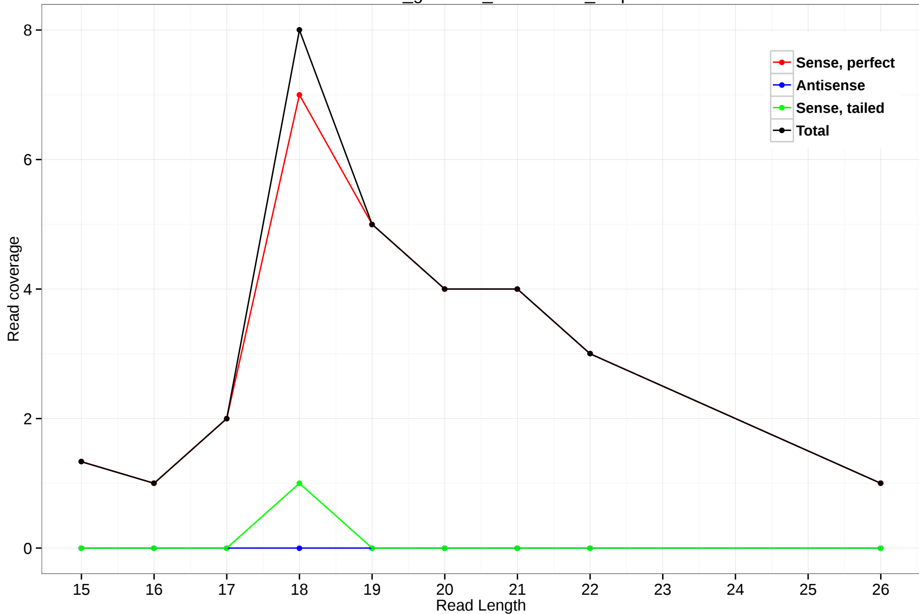
rheMac3_genscan_chr10.1661_0.5p
