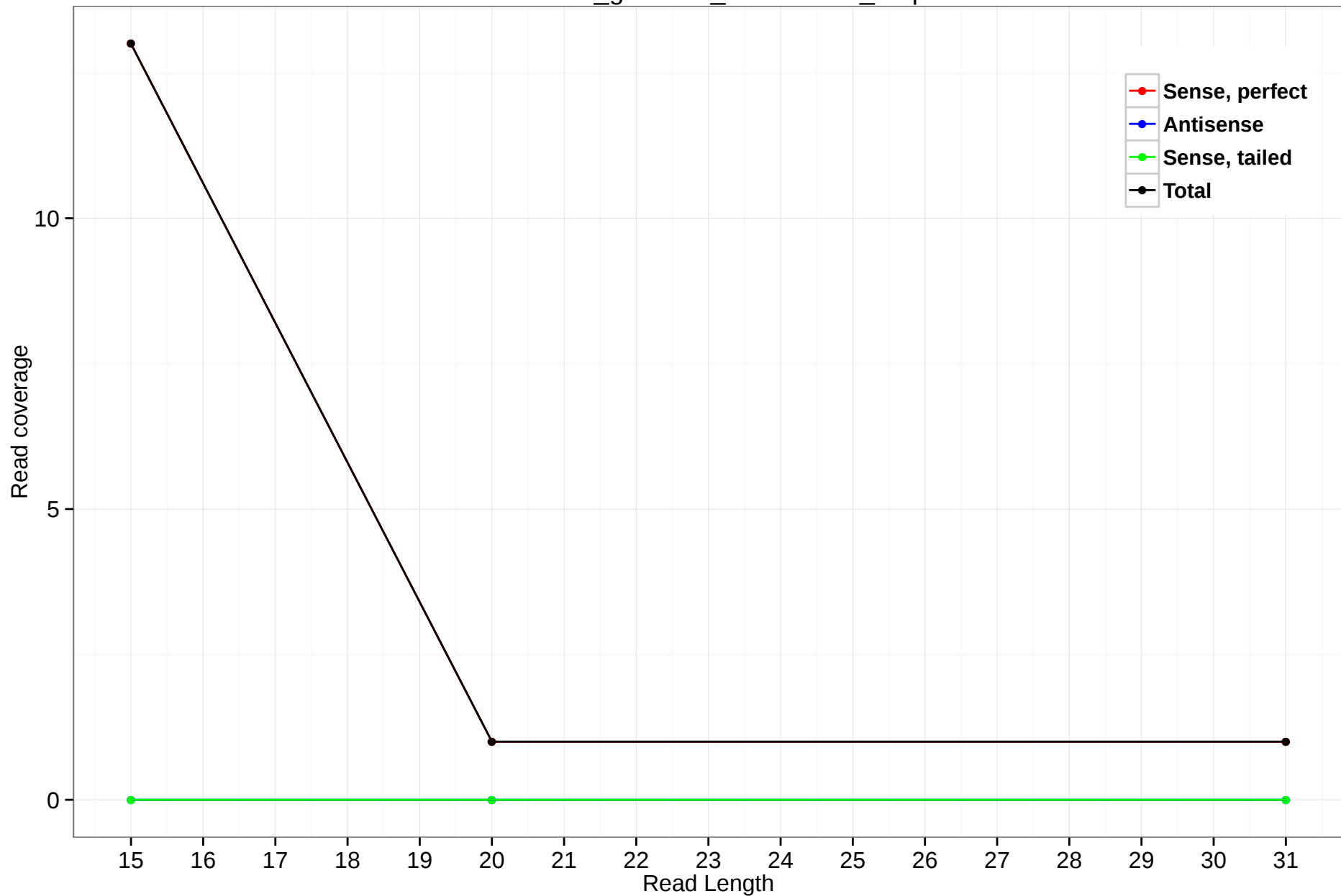
rheMac3_genscan_chr10.1660_7.5p
