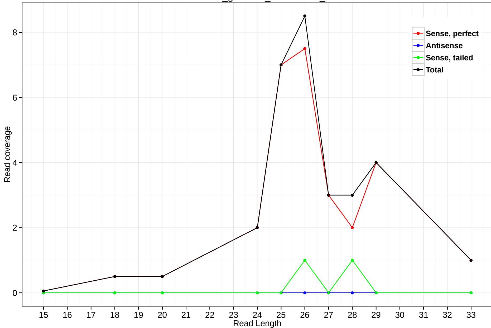
rheMac3_genscan_chr10.1659_3
