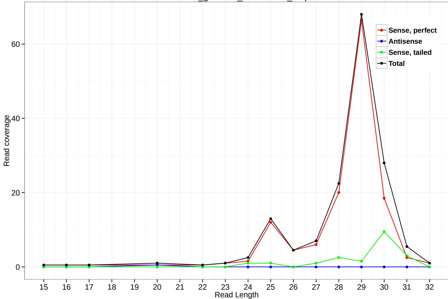
rheMac3_genscan_chr10.1656_6.5p
