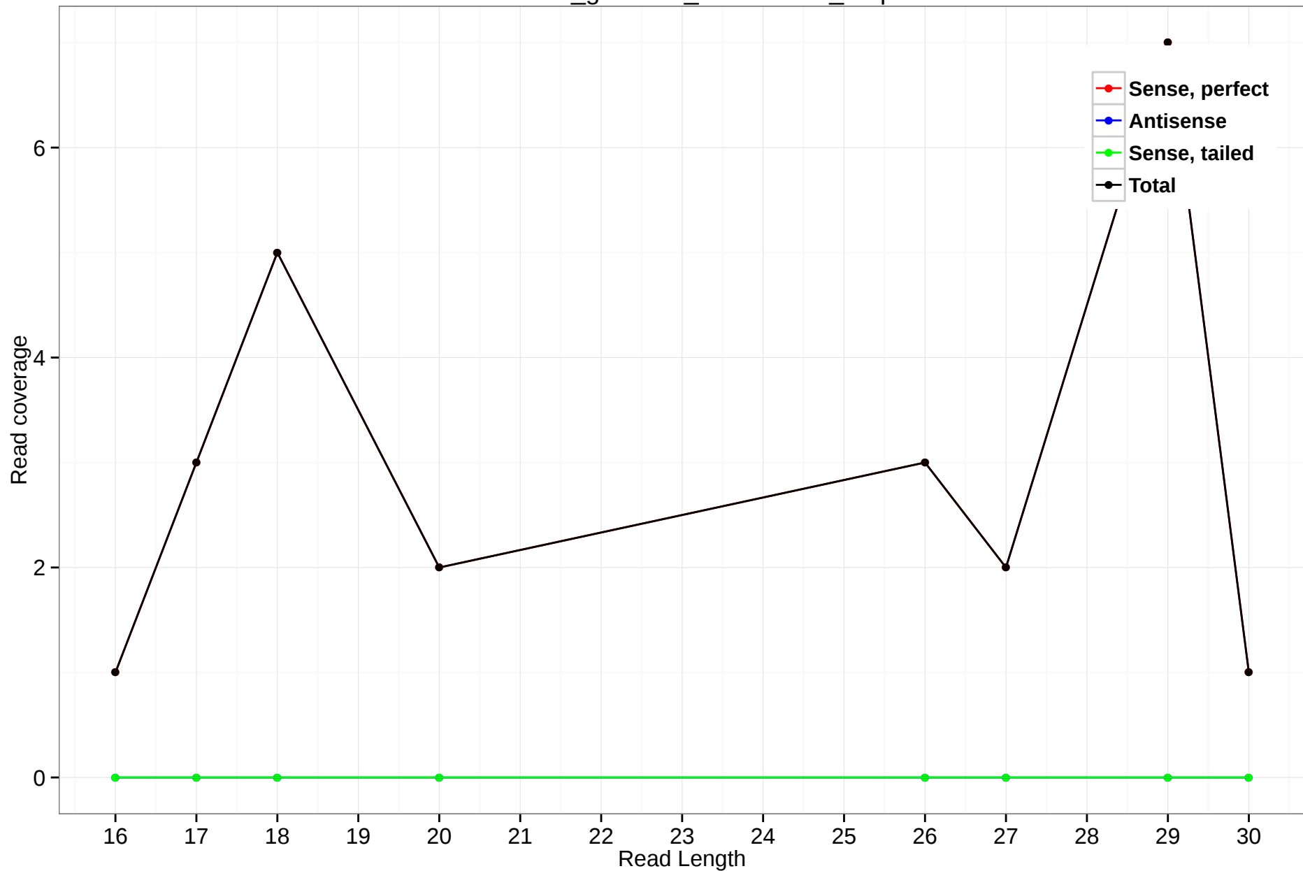
rheMac3_genscan_chr10.1653_0.5p
