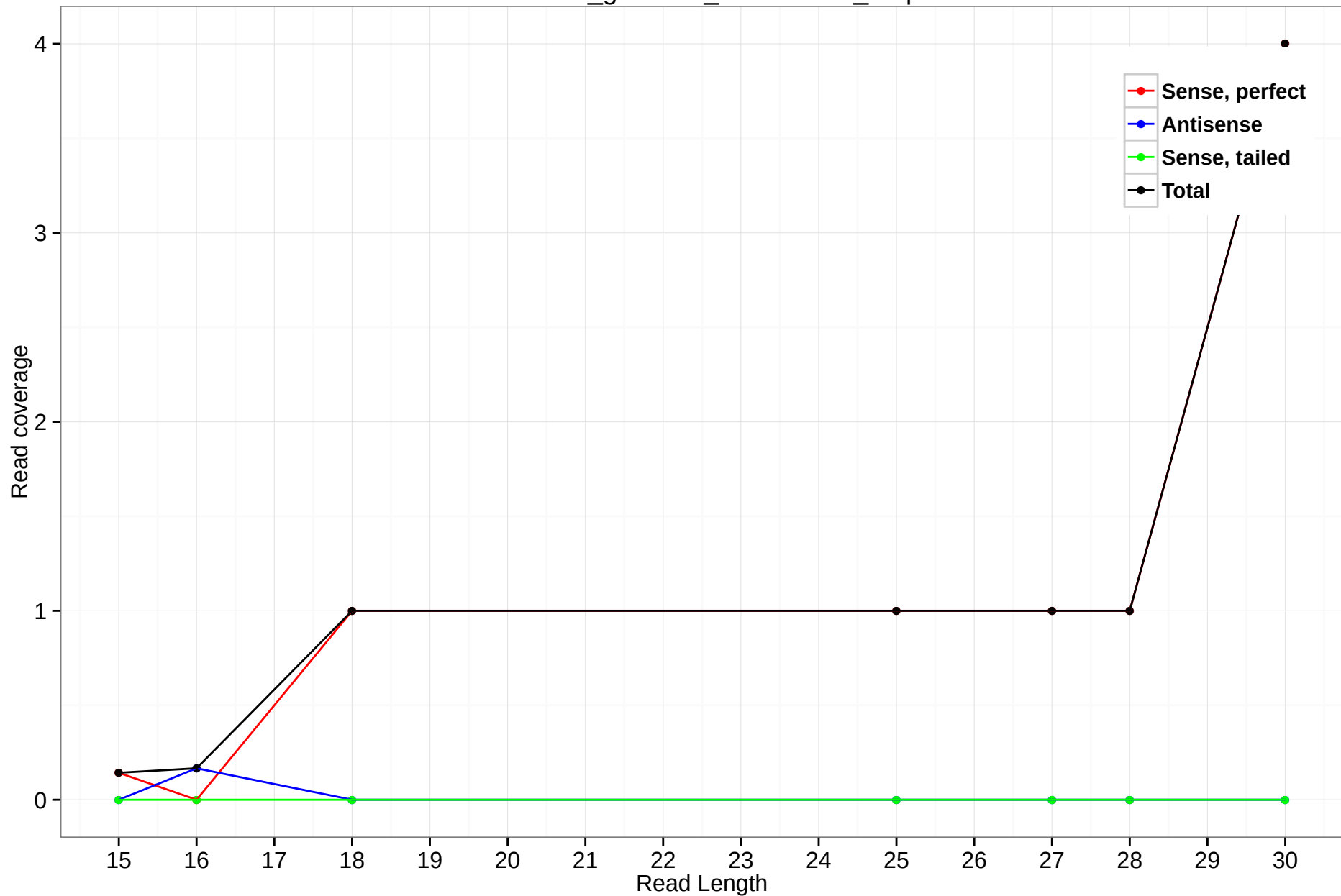
rheMac3_genscan_chr10.1650_6.5p
