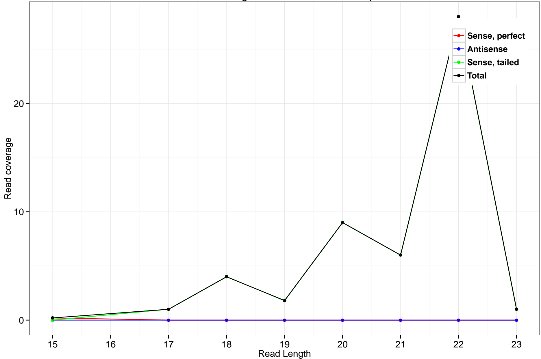
rheMac3_genscan_chr10.1627_19.5p
