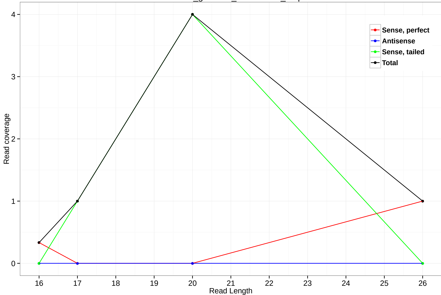
rheMac3_genscan_chr10.1599_9.3p
