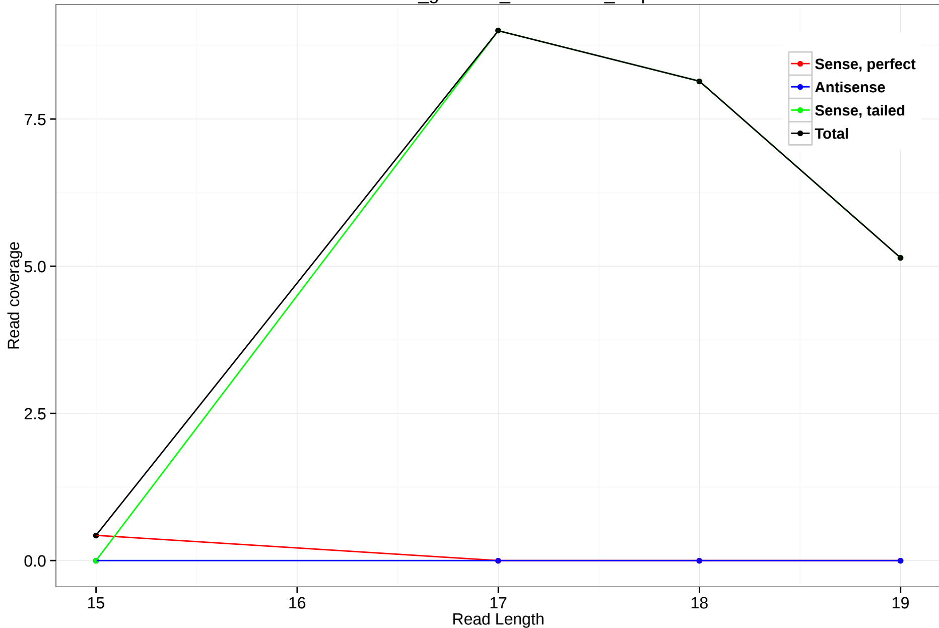
rheMac3_genscan_chr10.1599_7.5p
