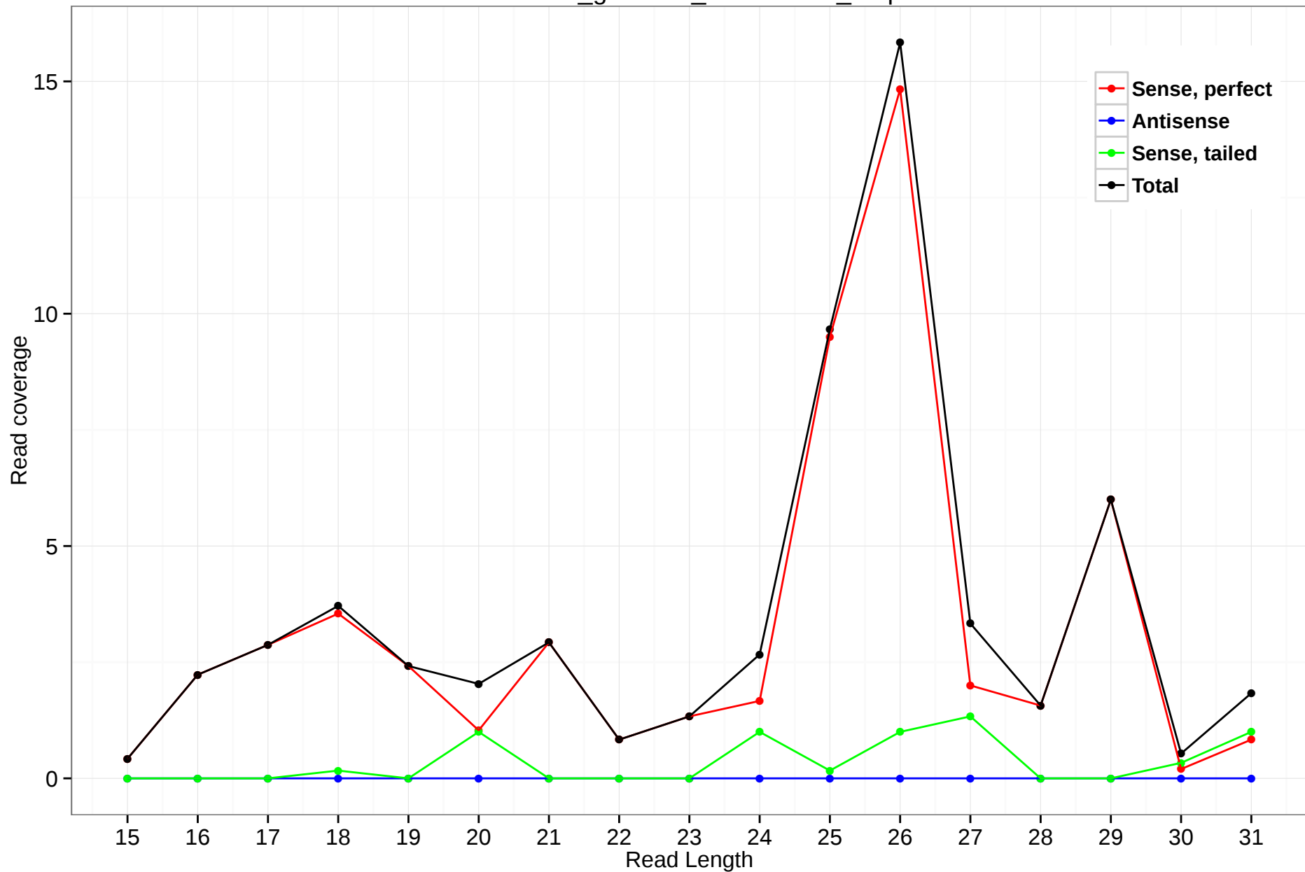
rheMac3_genscan_chr10.1598_0.3p
