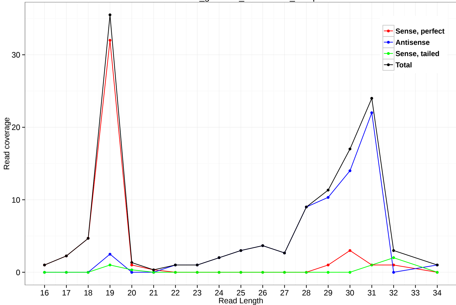
rheMac3_genscan_chr10.1580_53.5p
