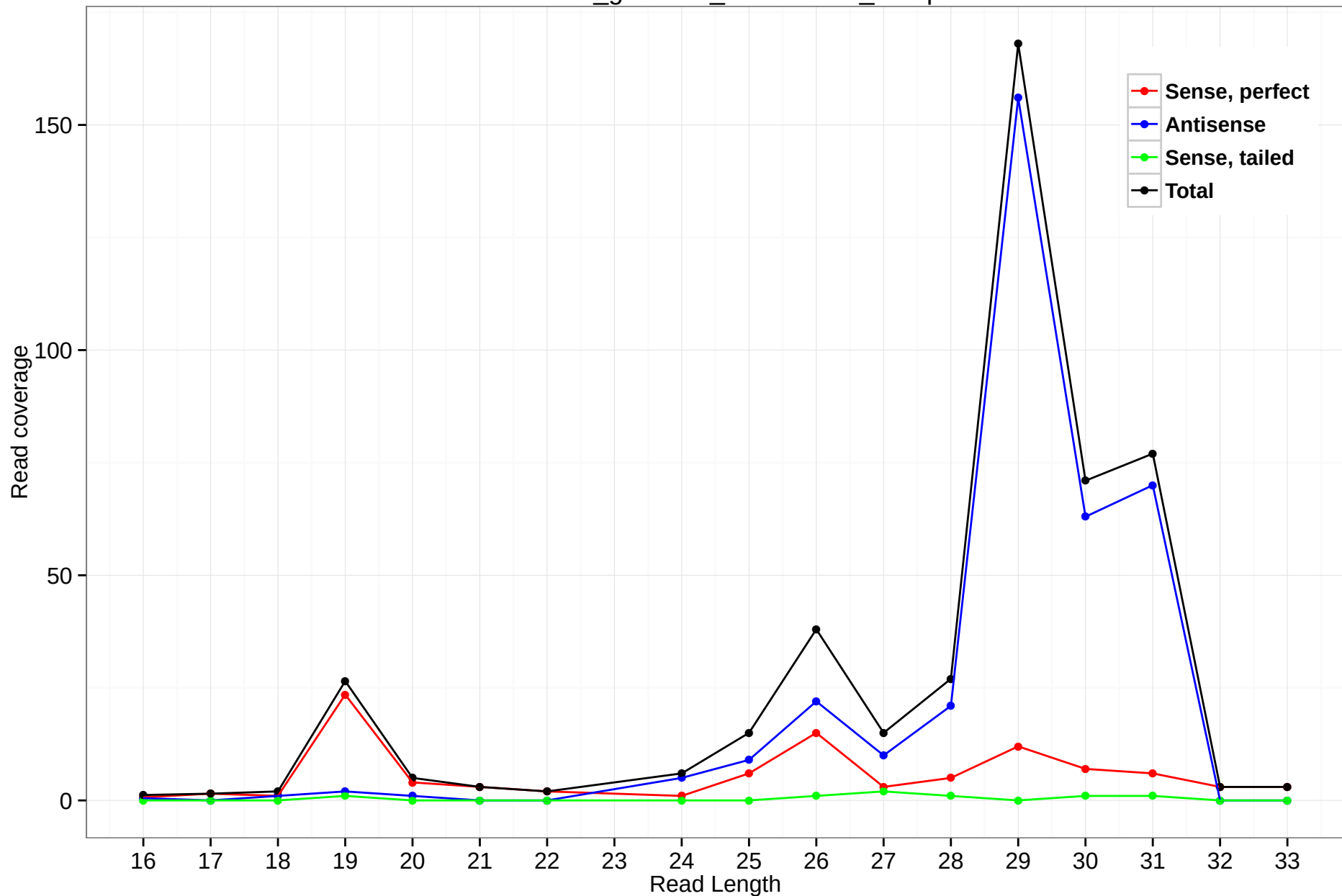
rheMac3_genscan_chr10.1580_49.5p
