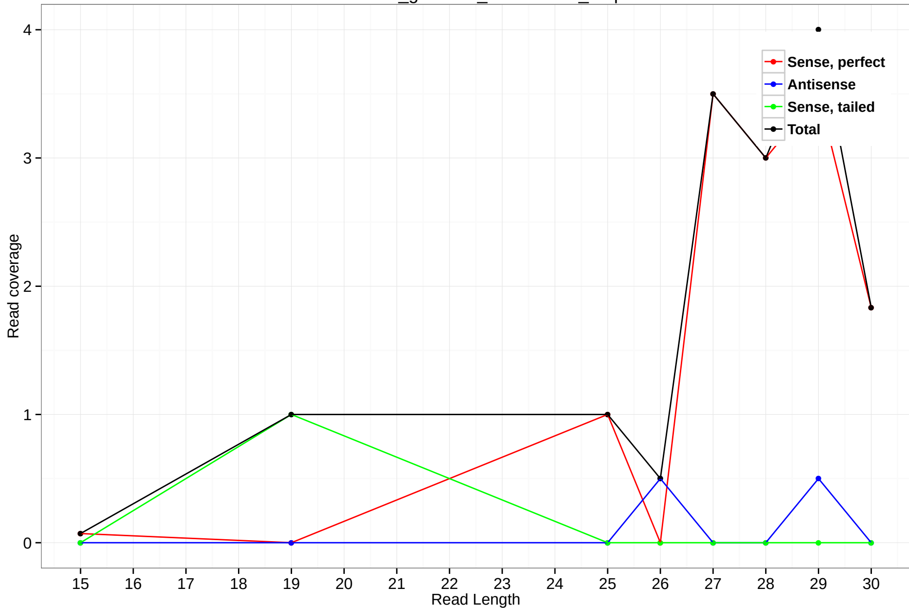
rheMac3_genscan_chr10.1570_8.5p
