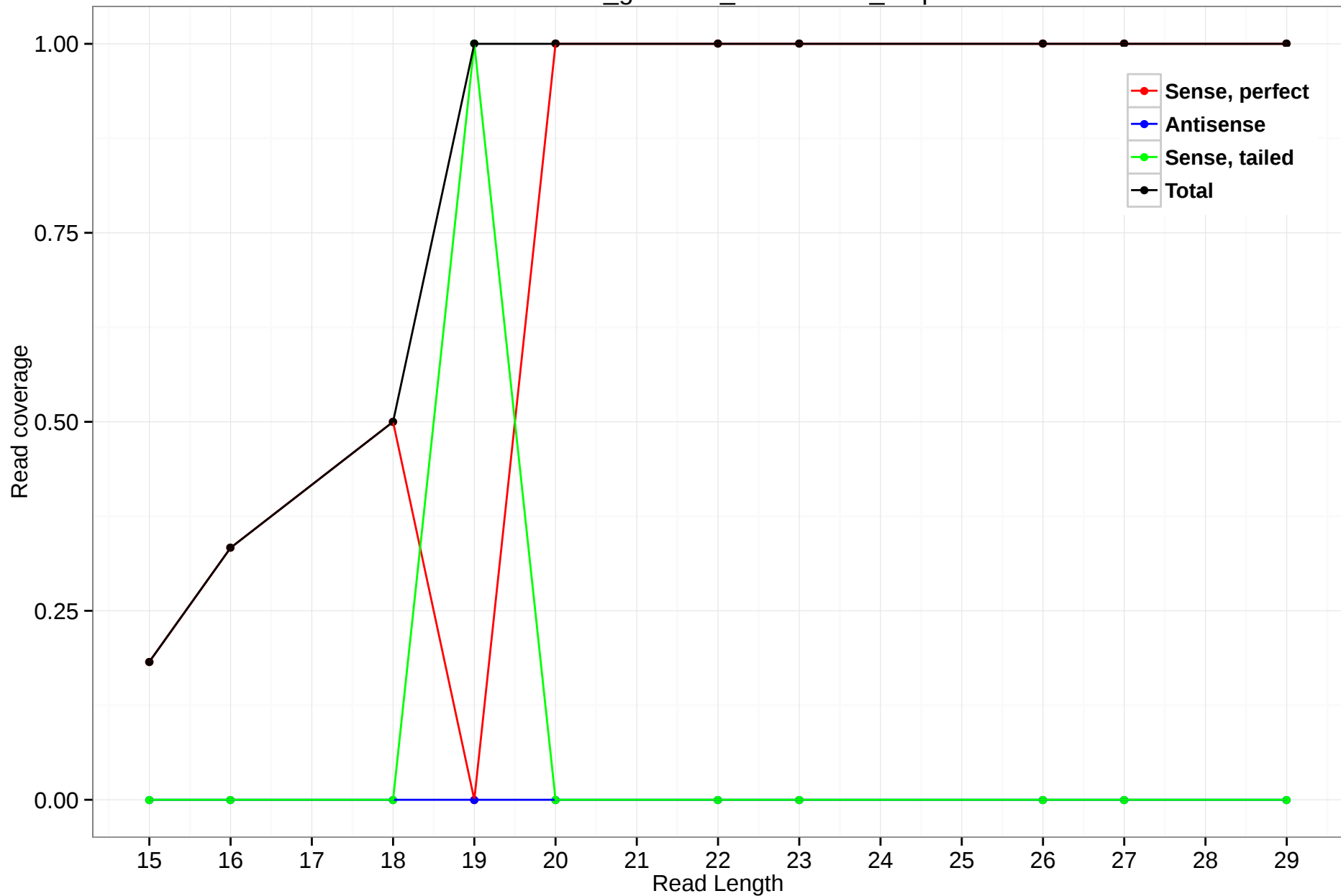
rheMac3_genscan_chr10.1570_5.5p
