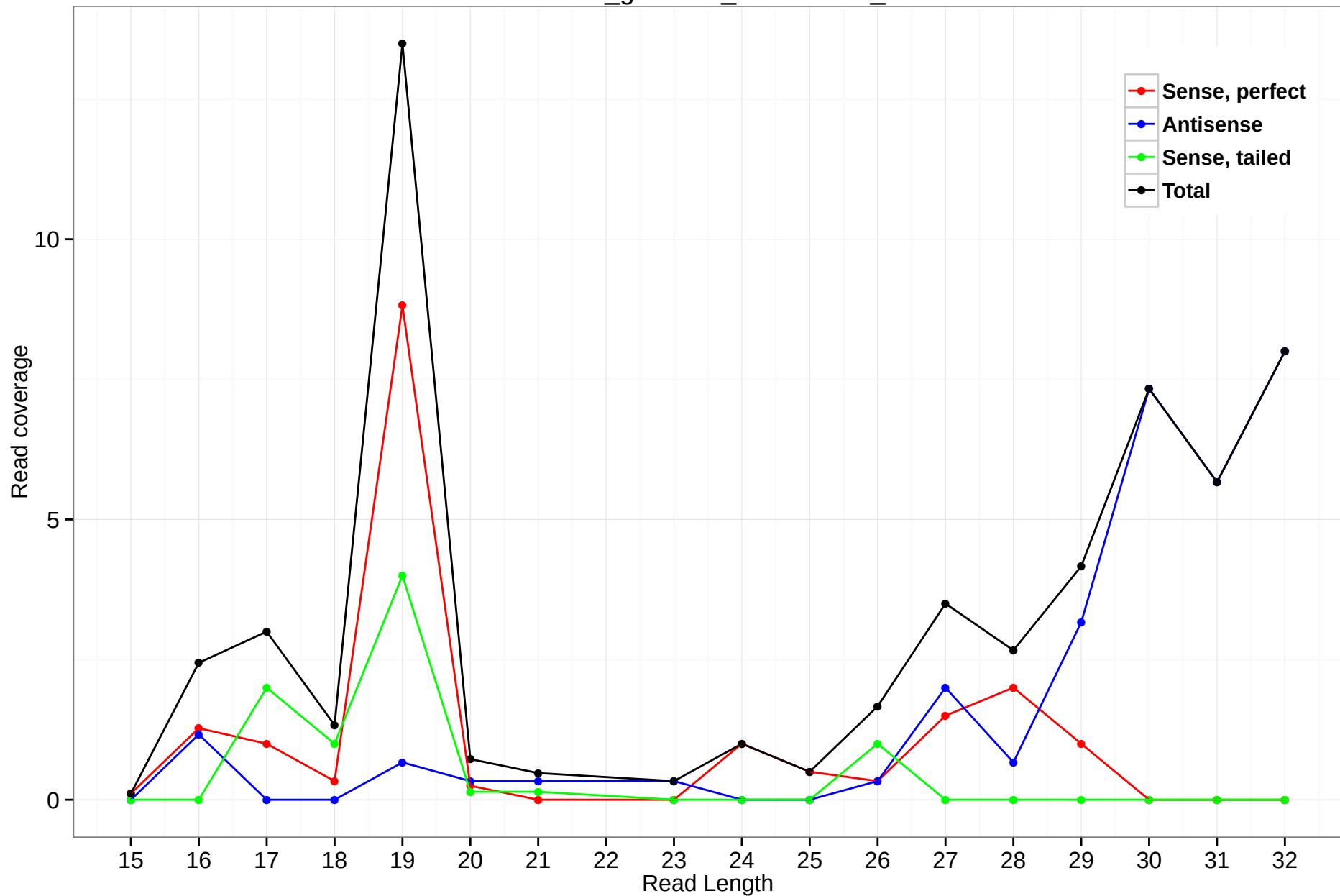
rheMac3_genscan_chr10.1570_11
