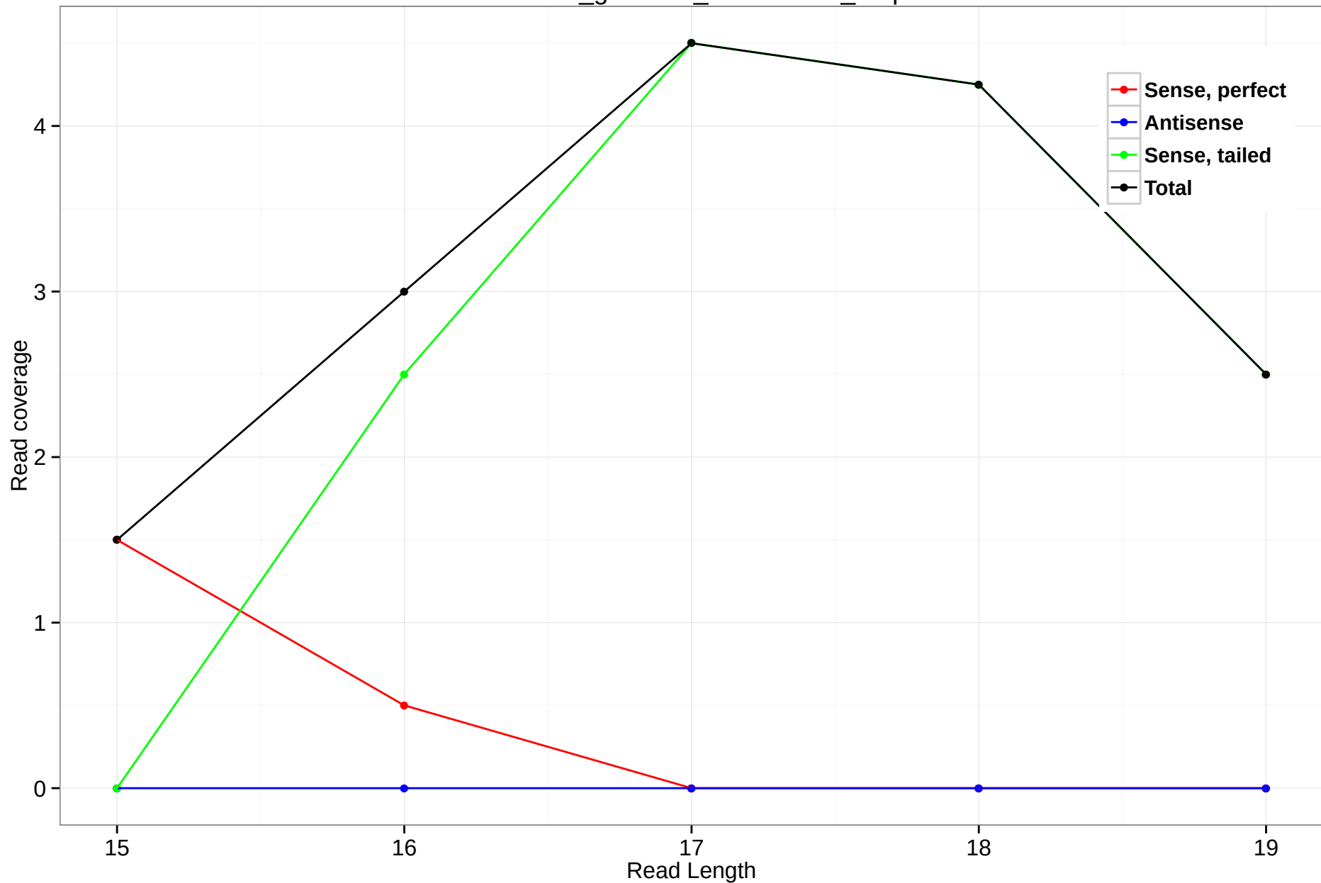
rheMac3_genscan_chr10.1566_2.5p
