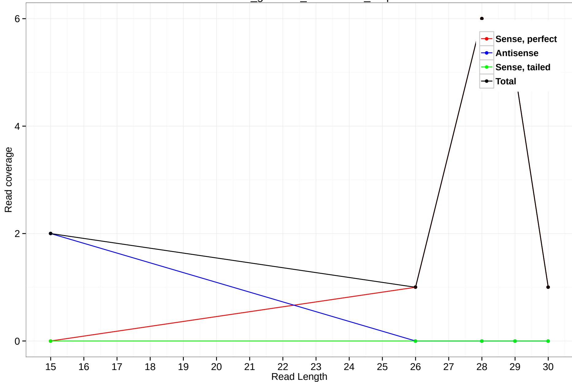
rheMac3_genscan_chr10.1562_3.5p
