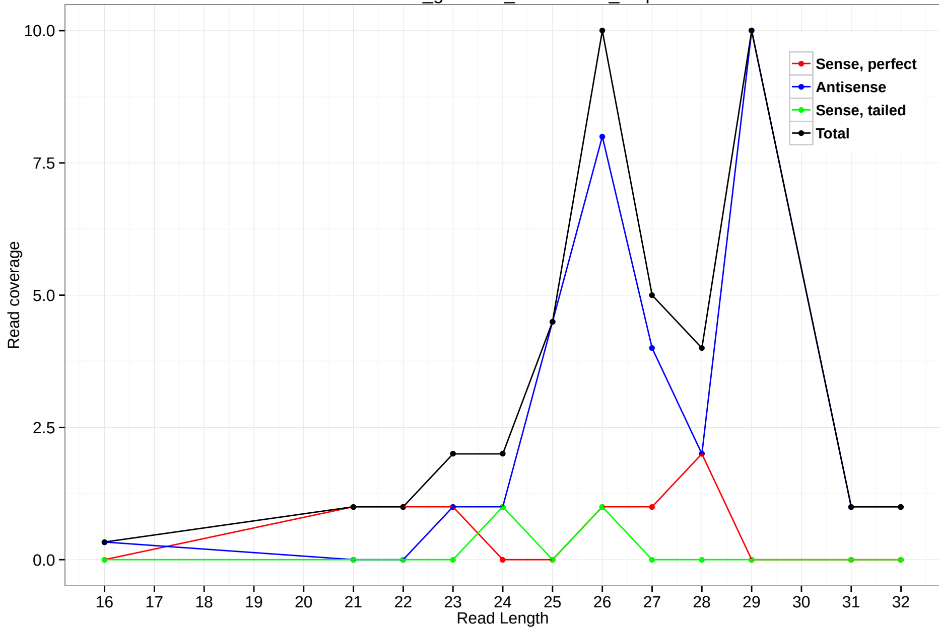
rheMac3_genscan_chr10.1554_1.5p
