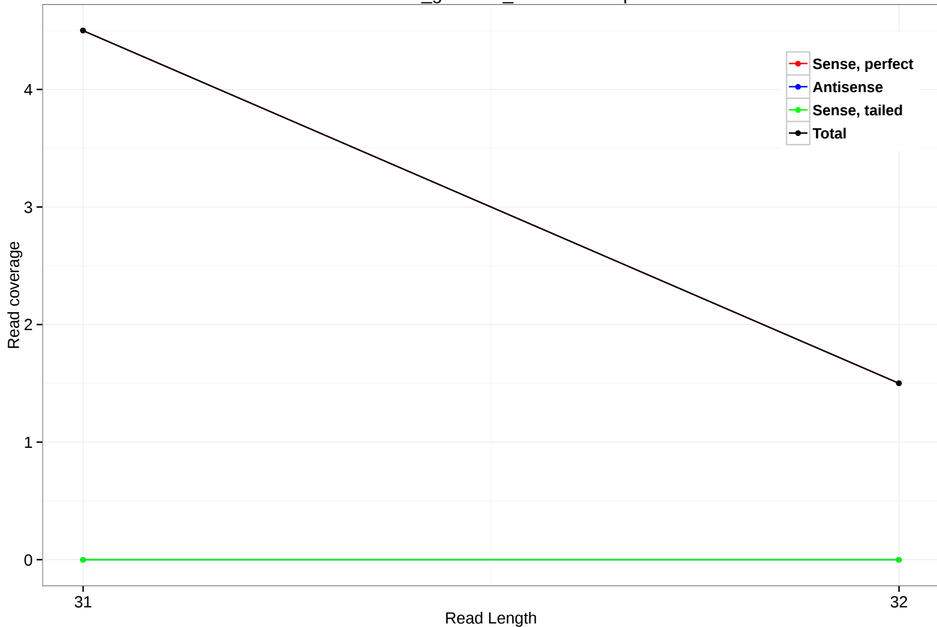
rheMac3_genscan_chr10.1529.5p
