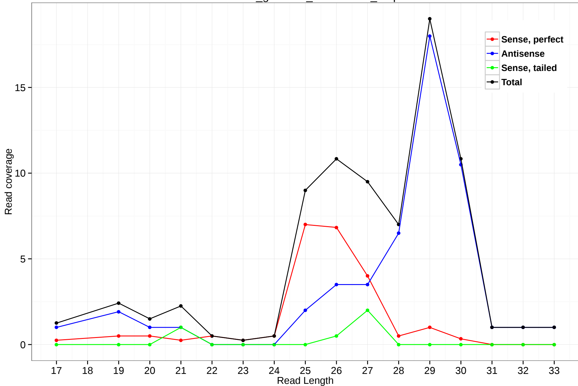
rheMac3_genscan_chr10.1522_9.3p
