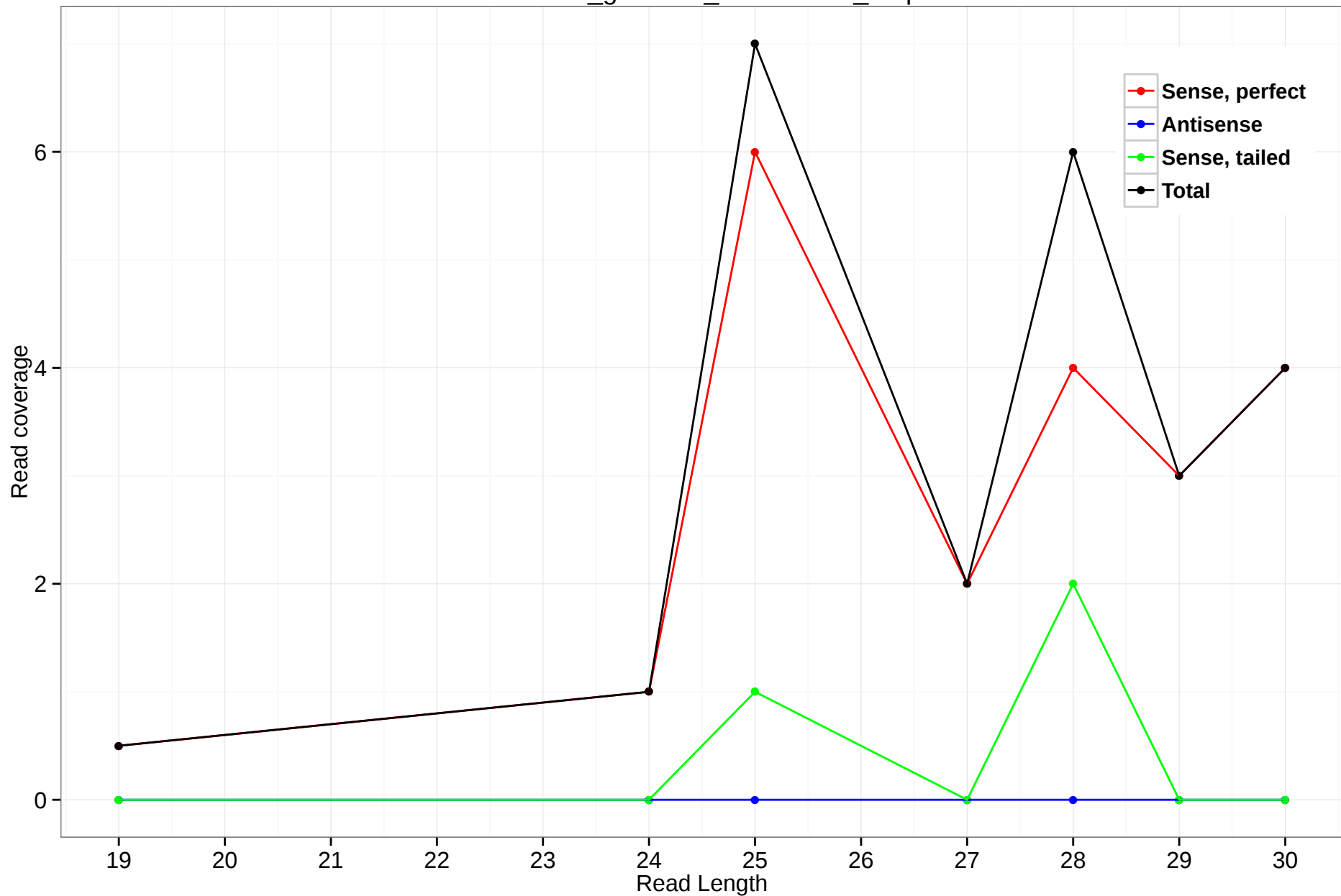
rheMac3_genscan_chr10.1522_5.3p
