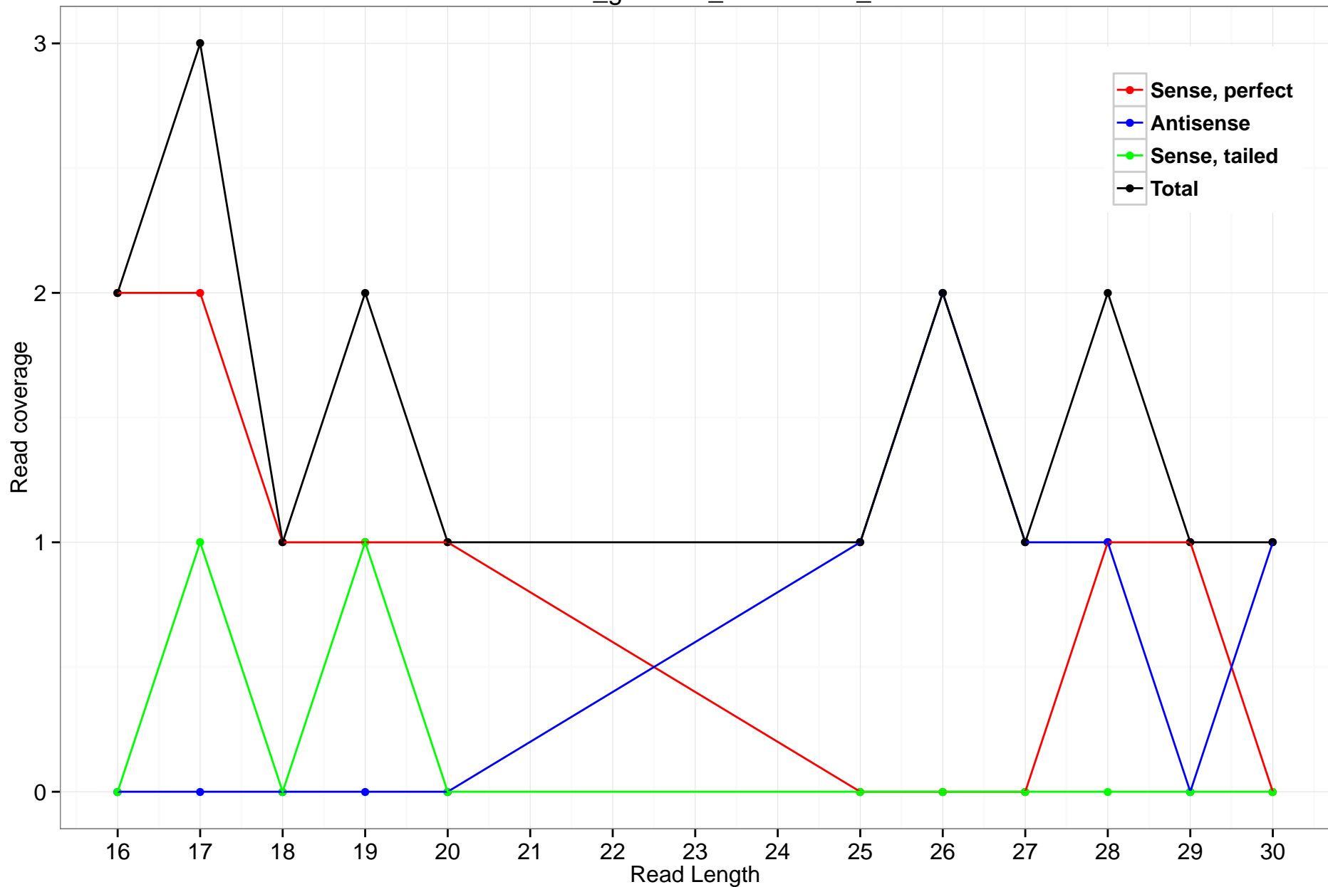
rheMac3_genscan_chr10.1509_23
