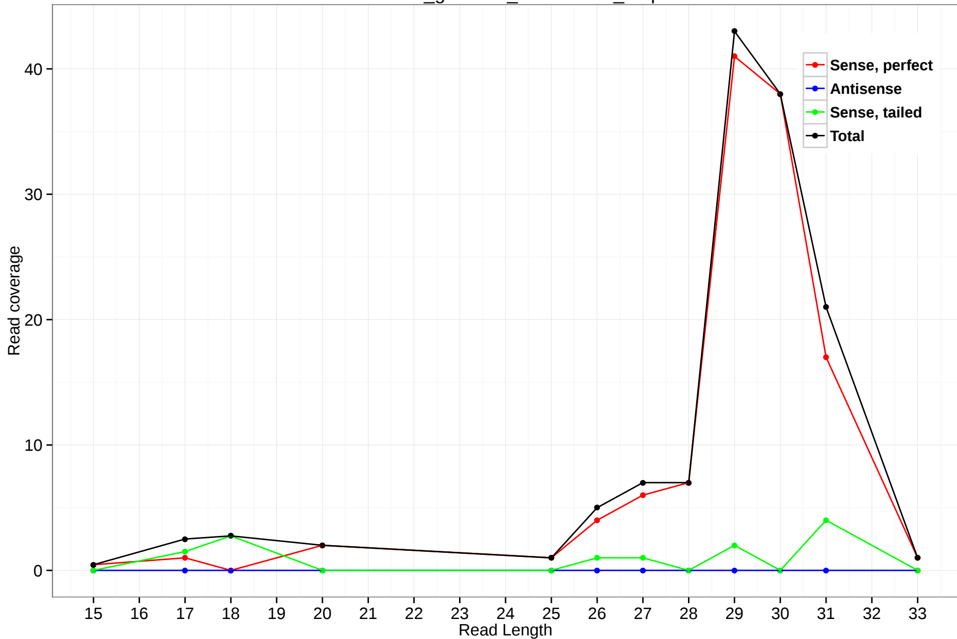
rheMac3_genscan_chr10.1497_2.3p
